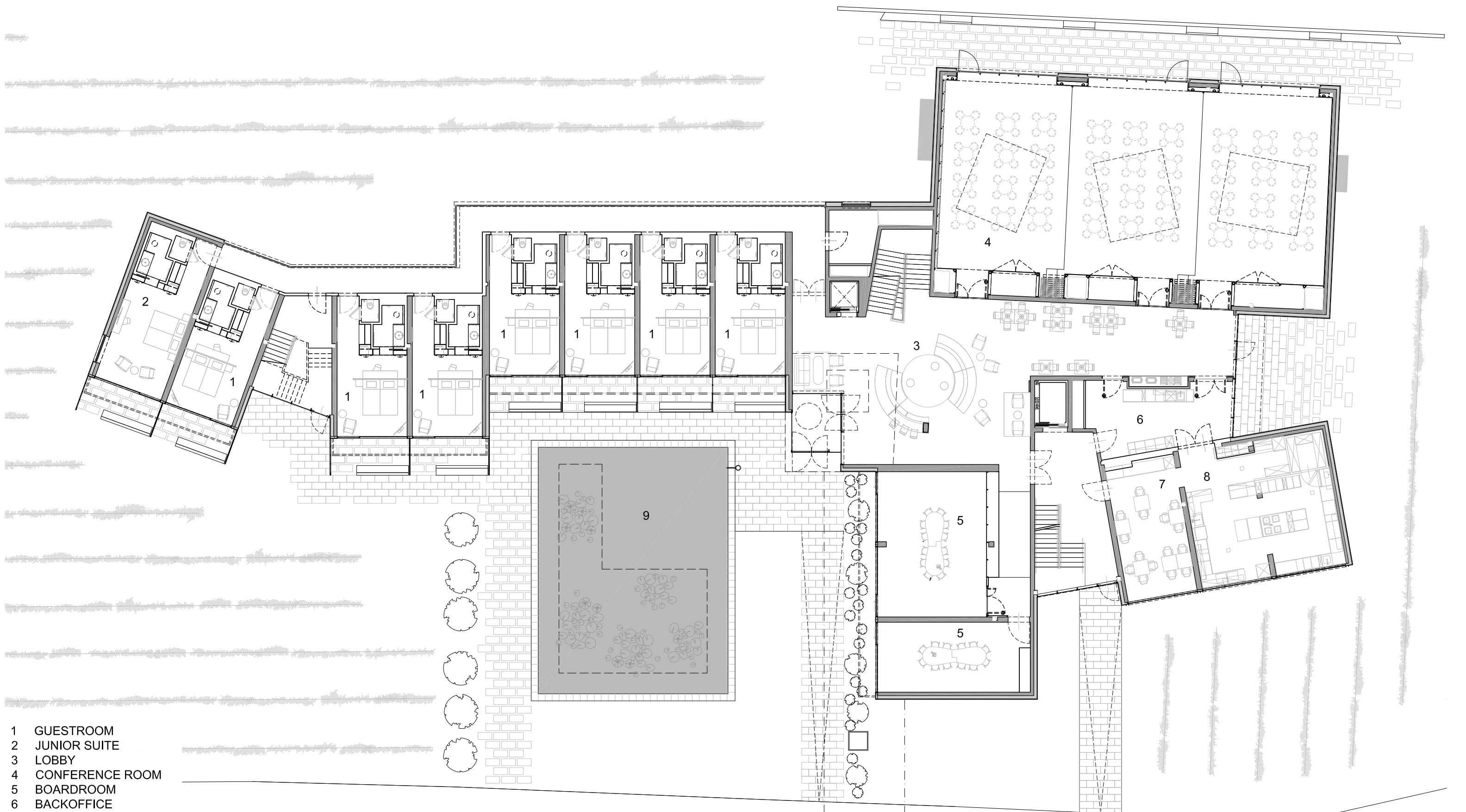
1st FL PLAN 1:200 0 1 5 10
