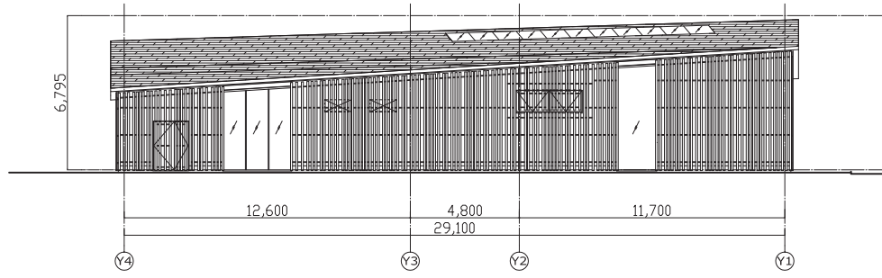
North 1:300
