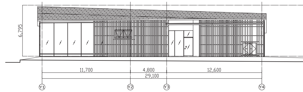
South 1:300
