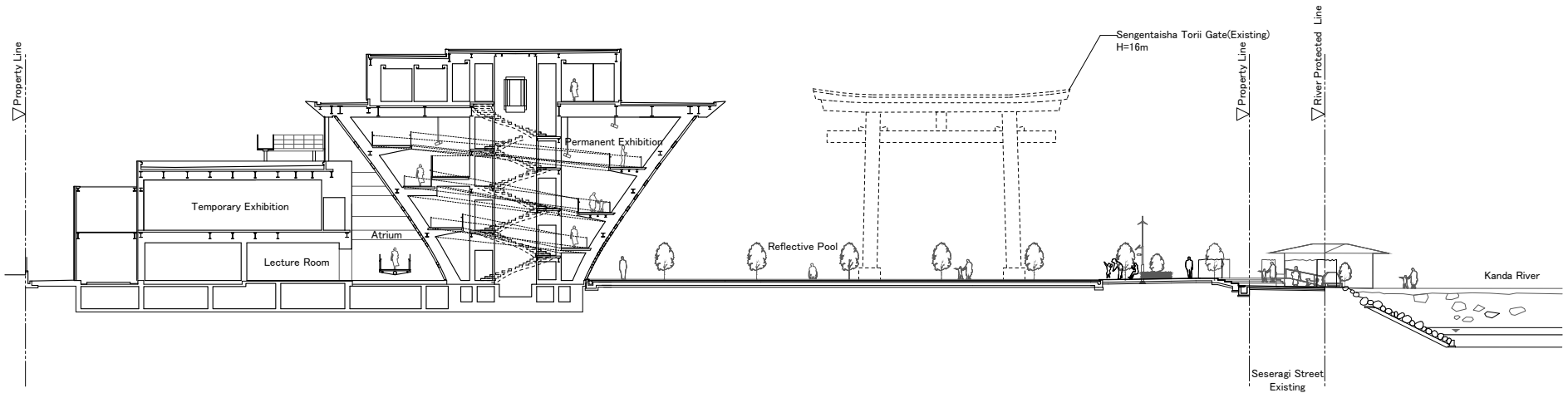
B-B' Short Section 1:500
