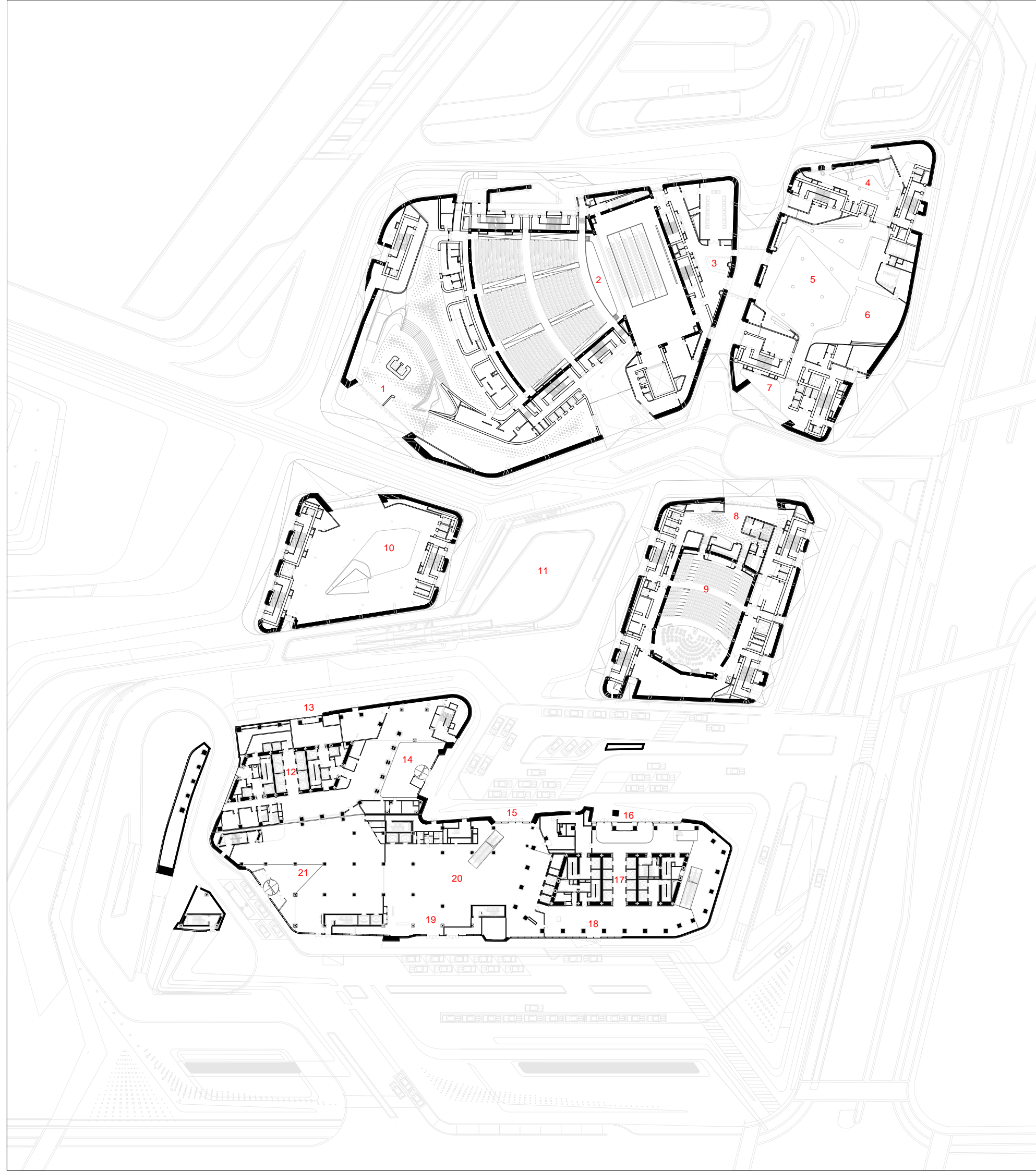
GROUND FLOOR PLAN Nanjing International Youth Cultural Centre
