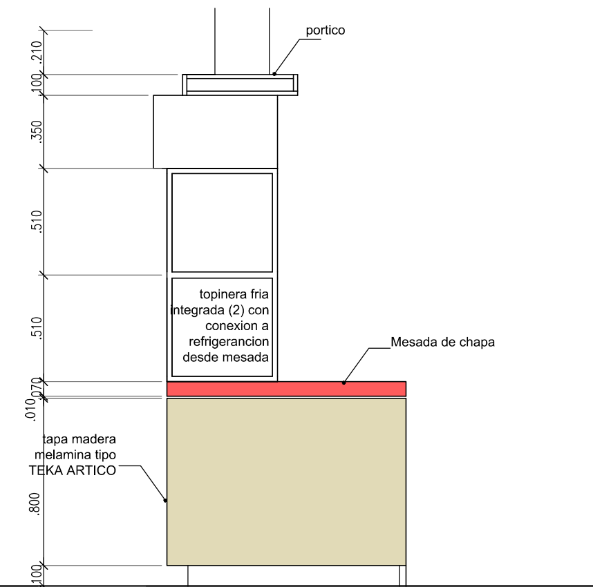
VISTA 4 (LATERAL)
