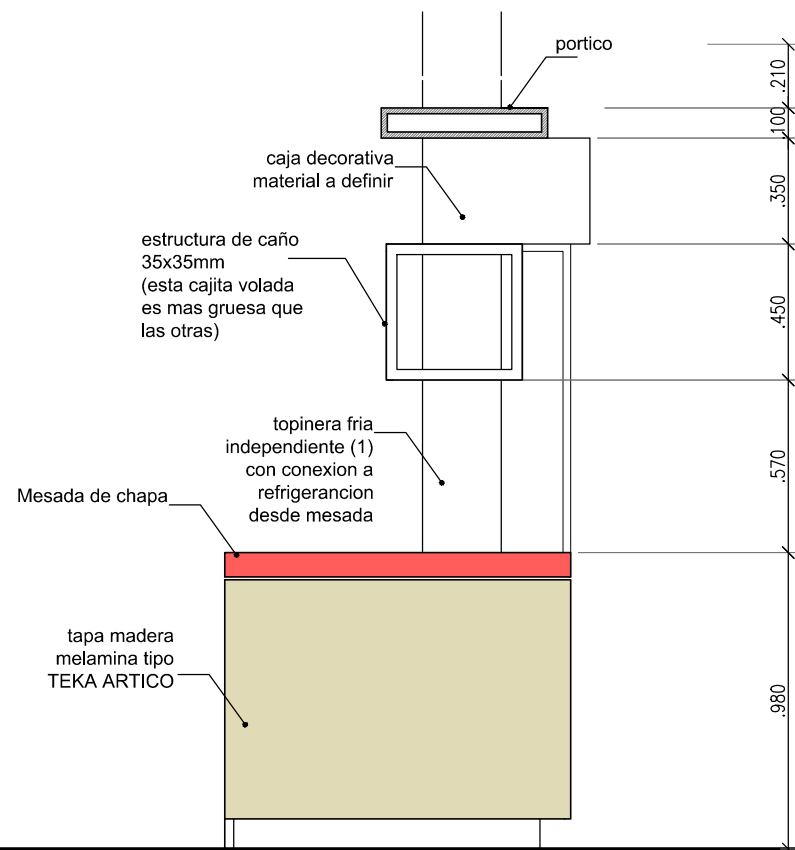
VISTA 3 (LATERAL)
