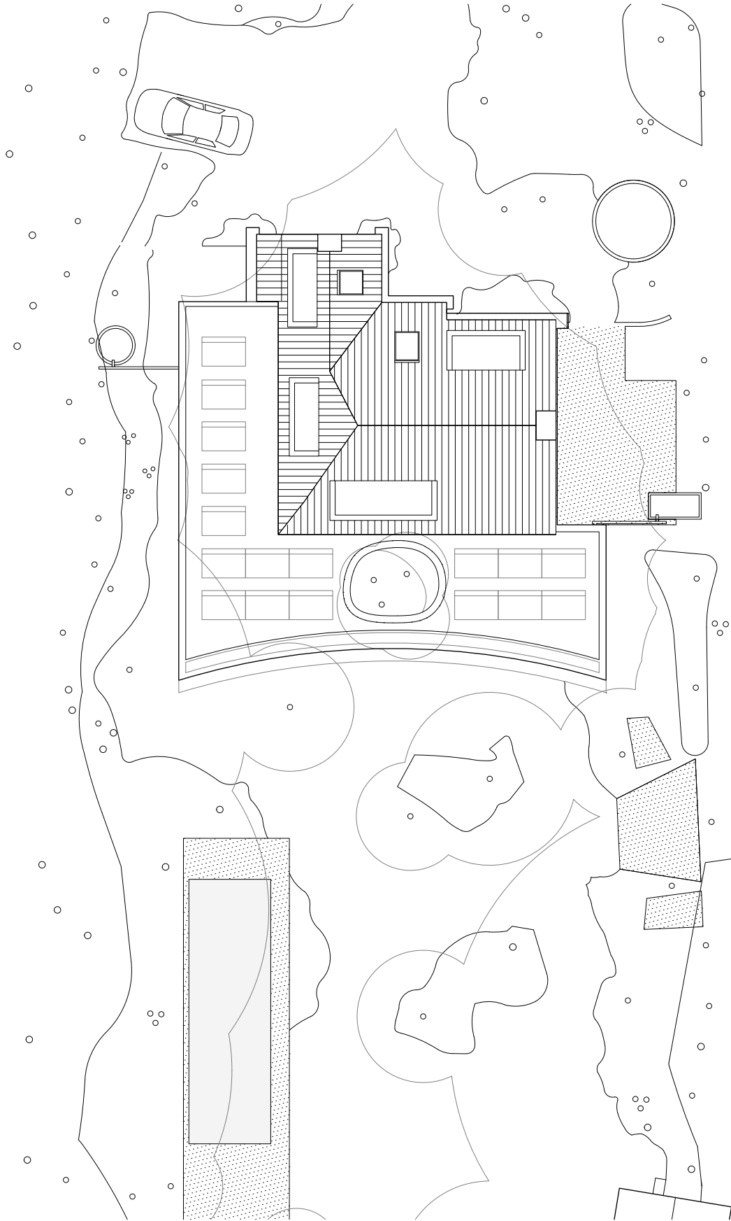
ROOF PLAN
