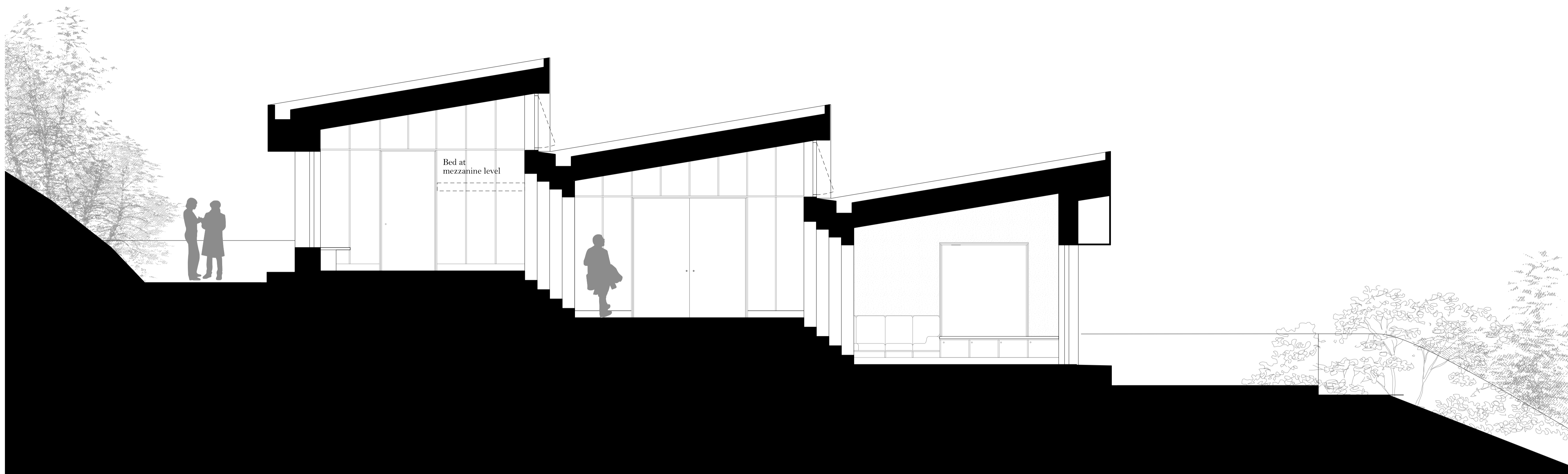
Section AA
