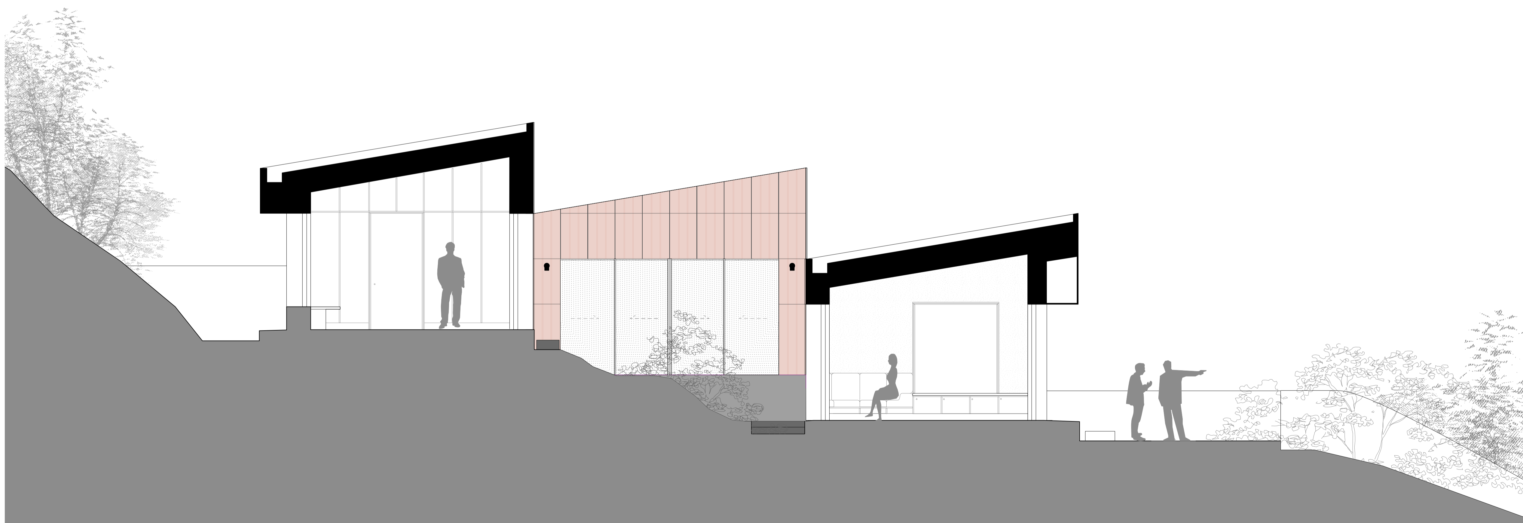
Section BB
