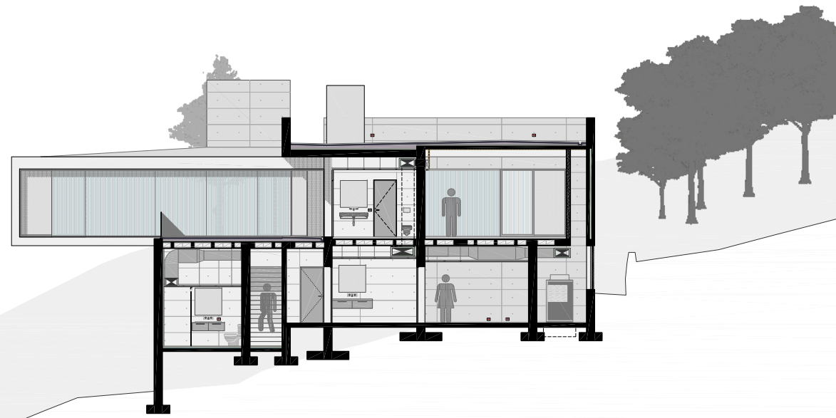
SECTION C
