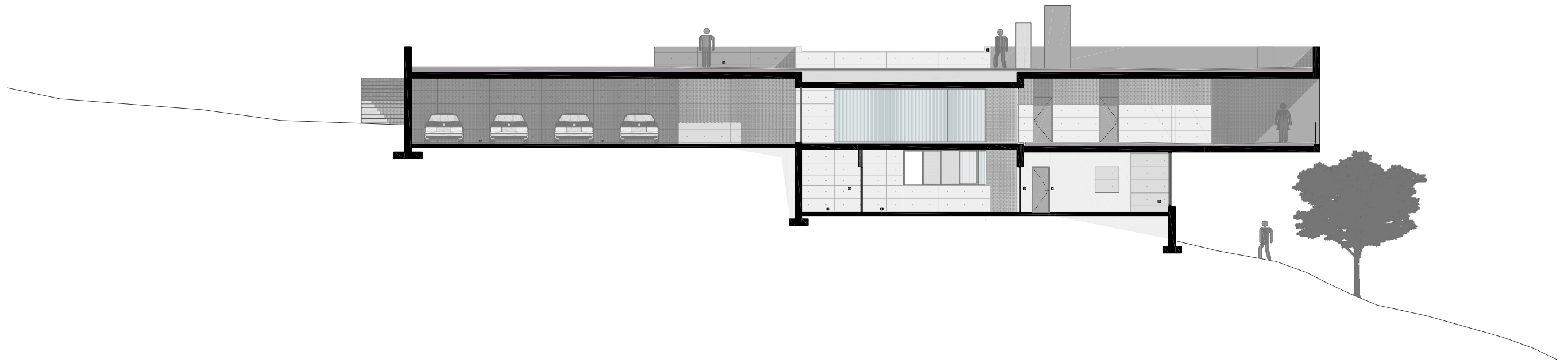
SECTION 3
