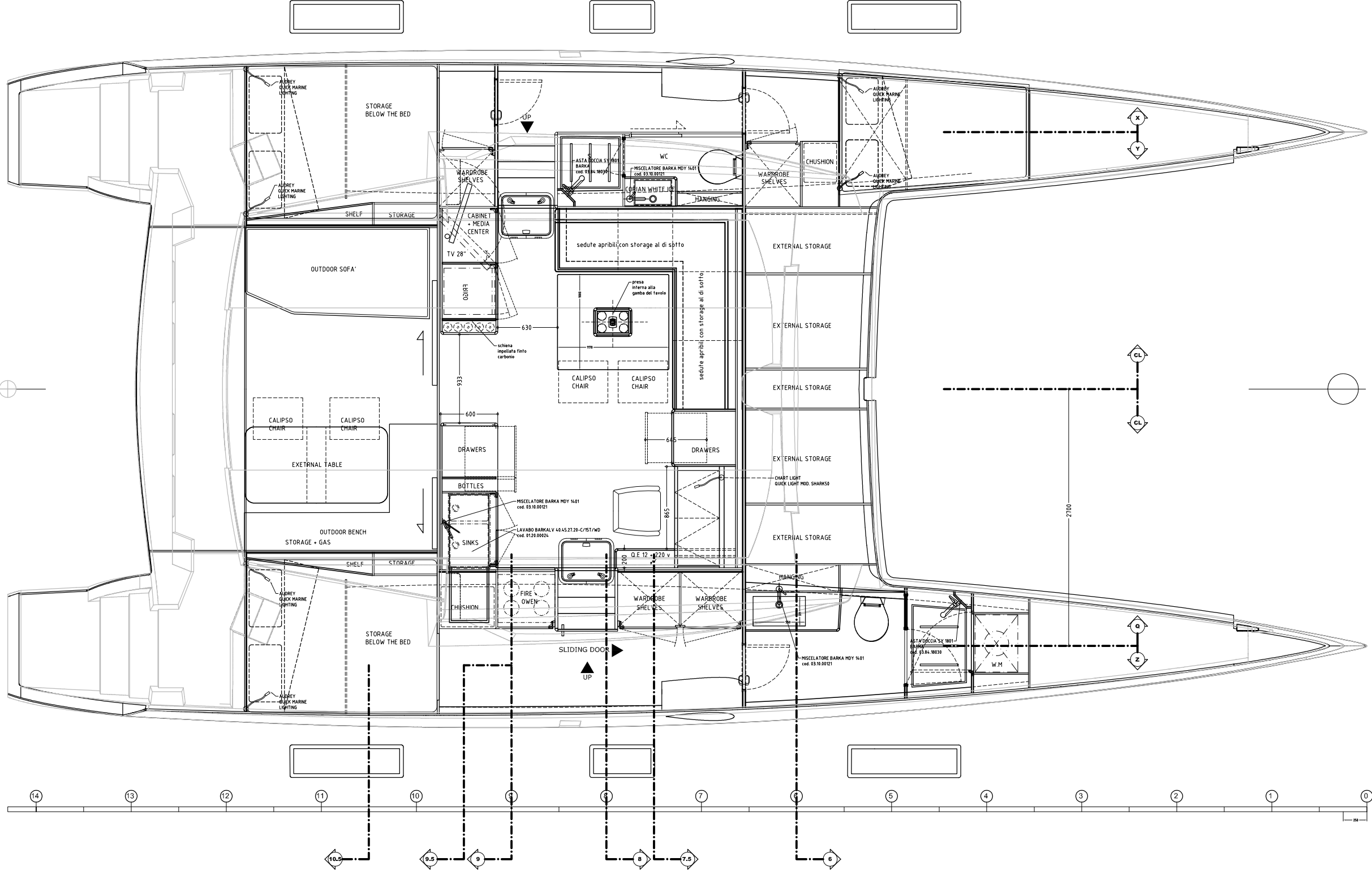
GENERAL ARRANGEMENT
