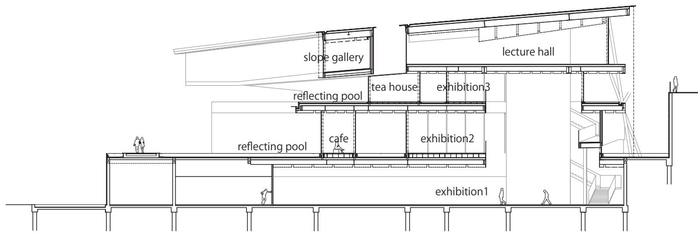
section 1 1/400
