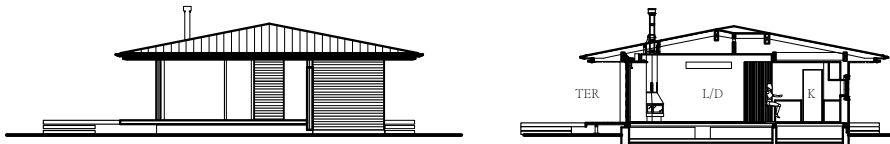
East Elevation S=1:150
