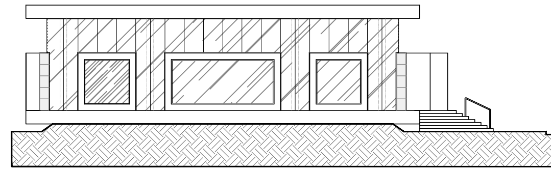
Elevation North-East
