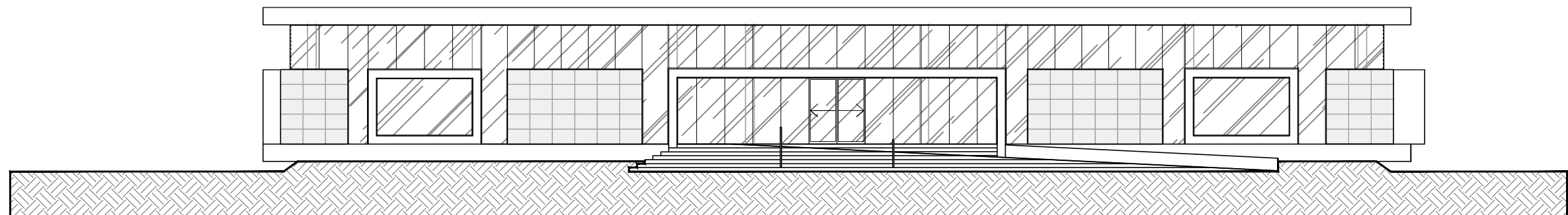
Elevation North-West
