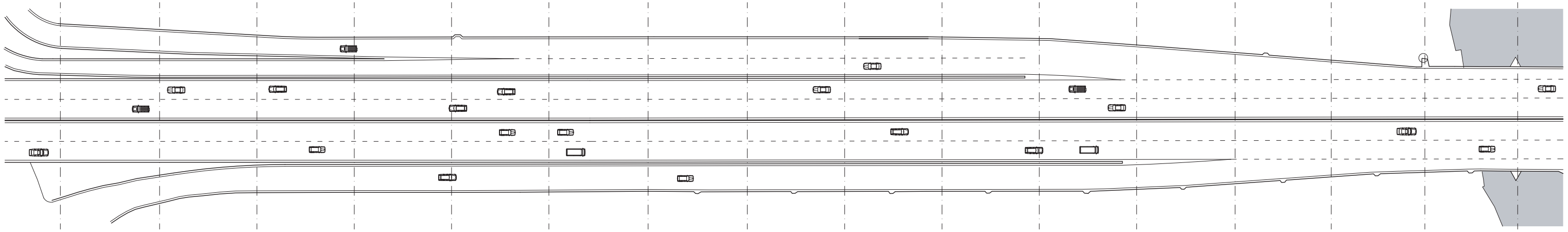
top view 1:1000
