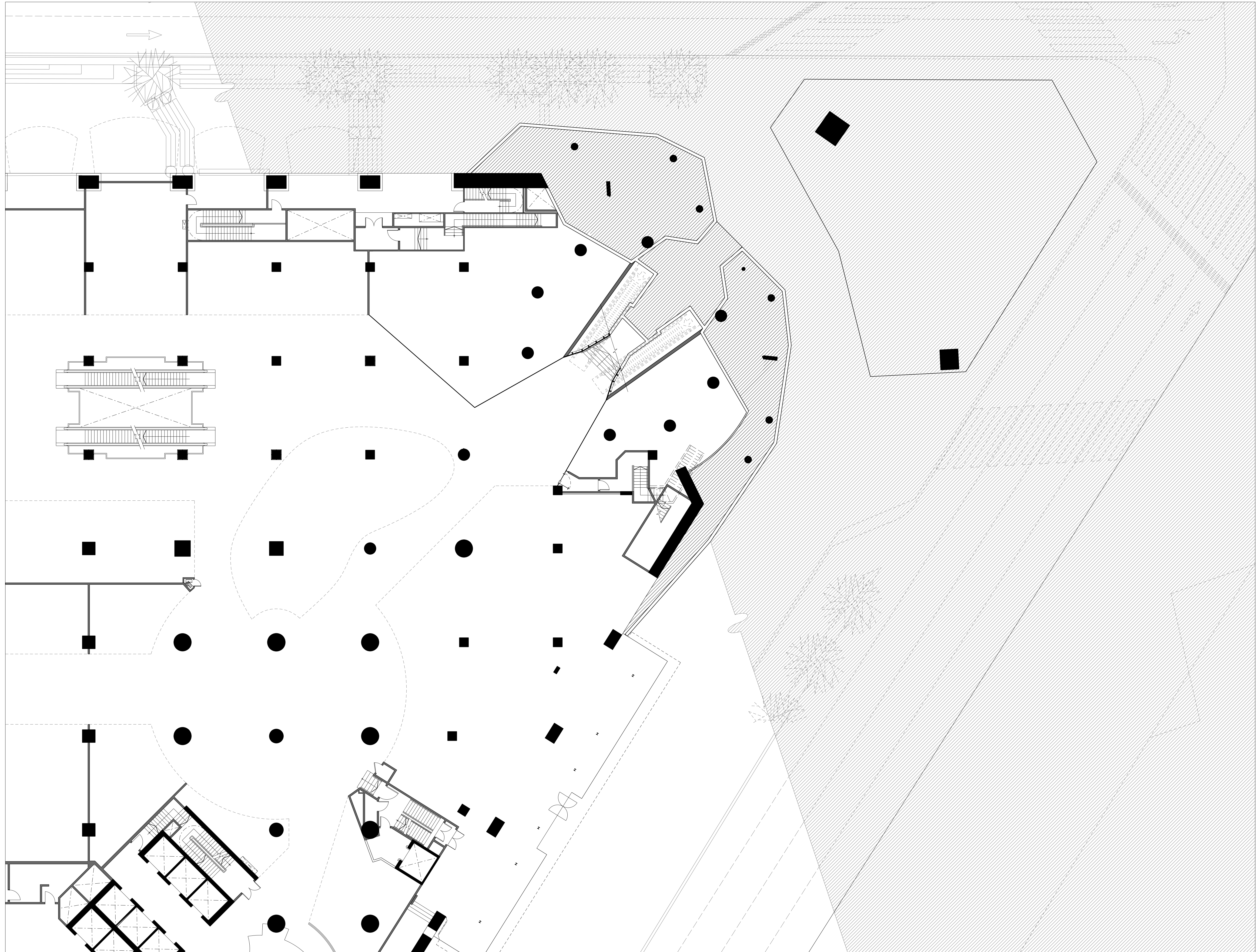
GA/p100 GENERAL ARRANGEMENT / PLAN LEVEL 2 SCALE 1:150
