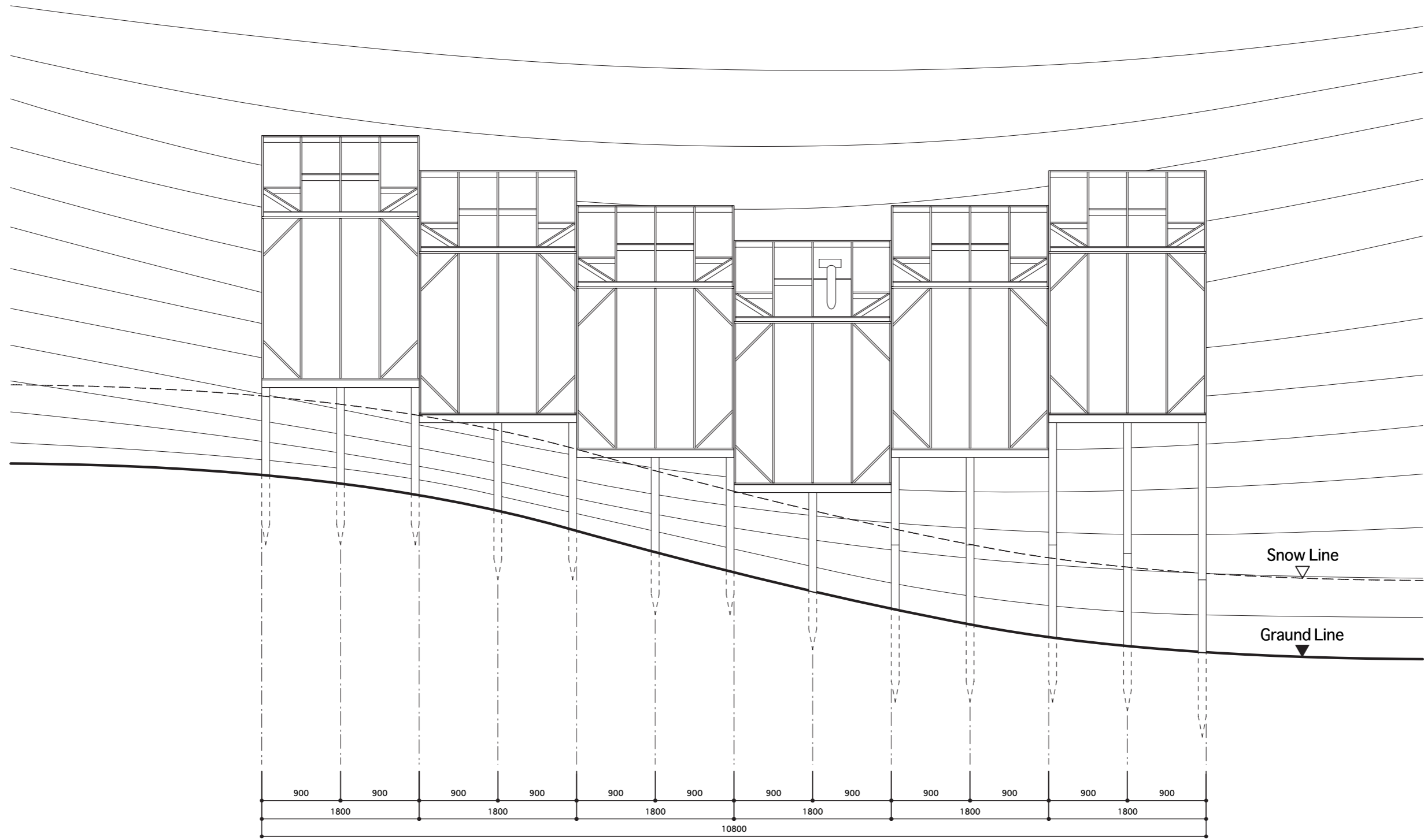
<WINTER HOUSE> East Elevation S=1/50
