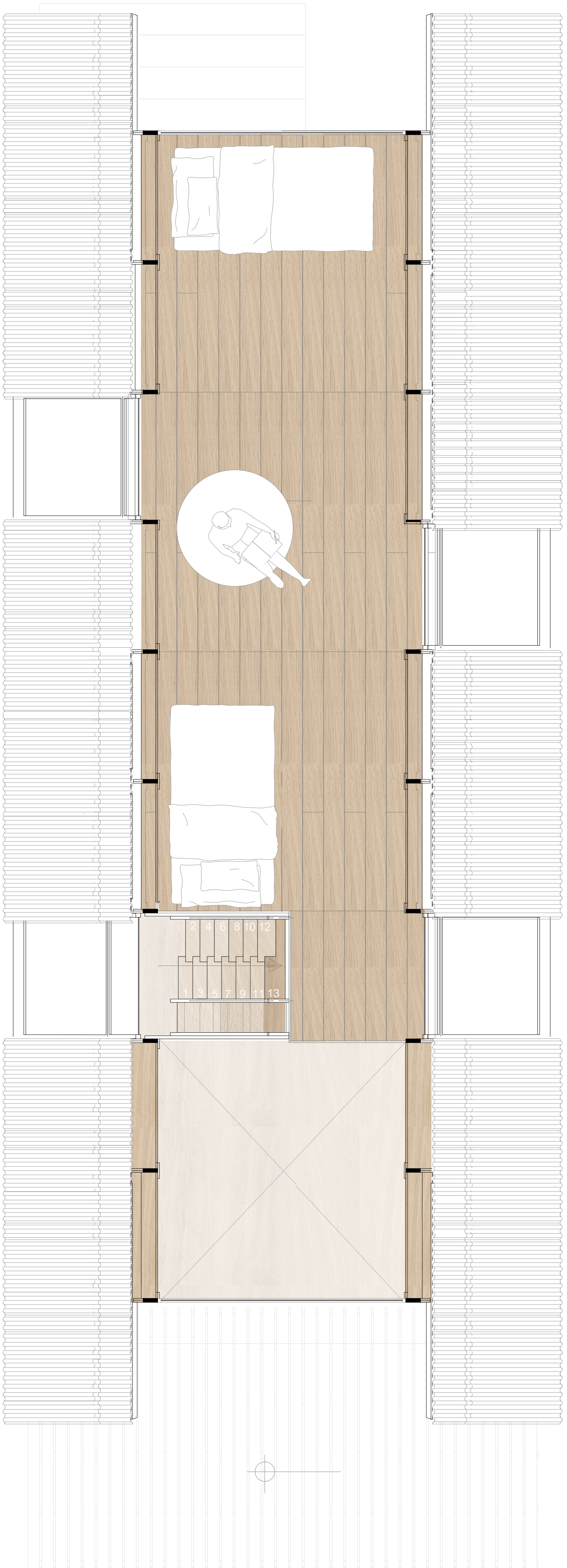
Planta Alta N+2.40
