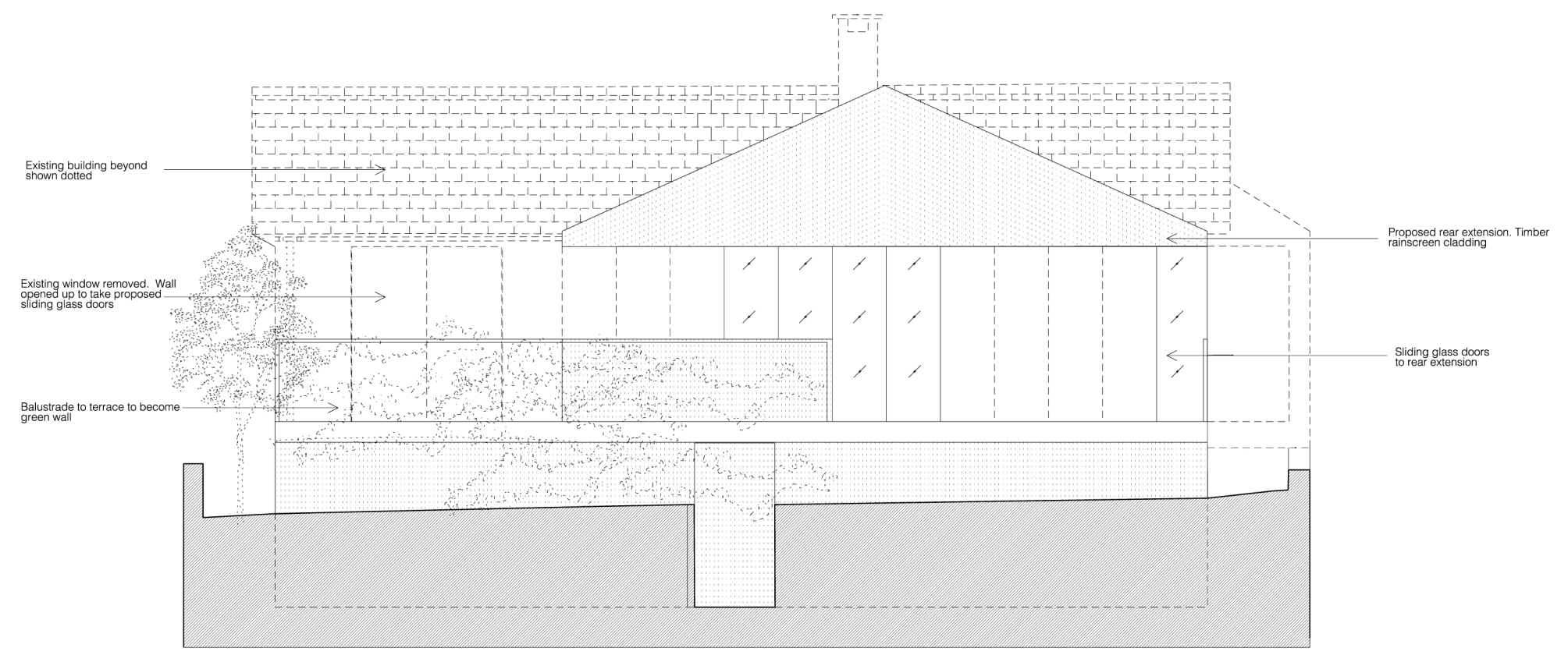
② Proposed South Elevation
