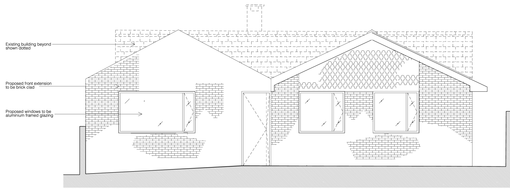
① Proposed North Elevation
