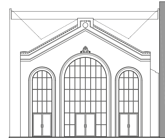
Facade 1:200
