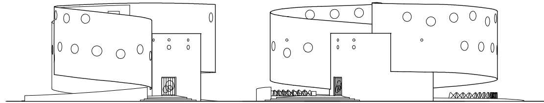
East Elevation S=1/400
