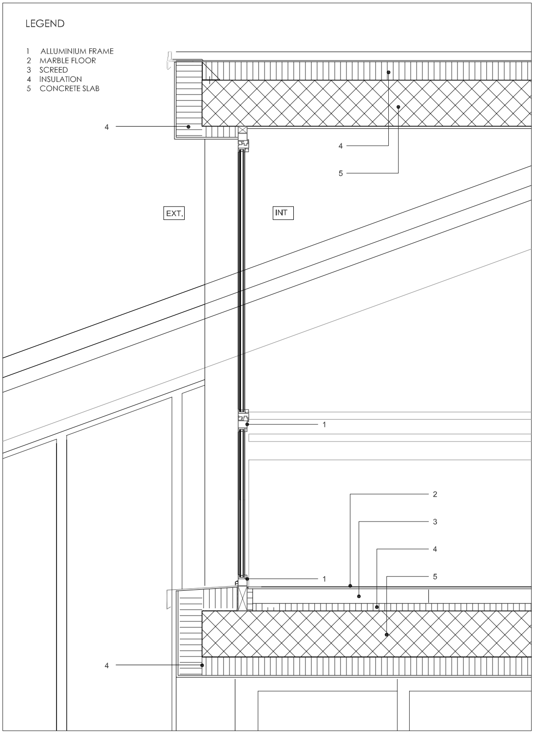
DETAIL 1 - SECTION VIEW
