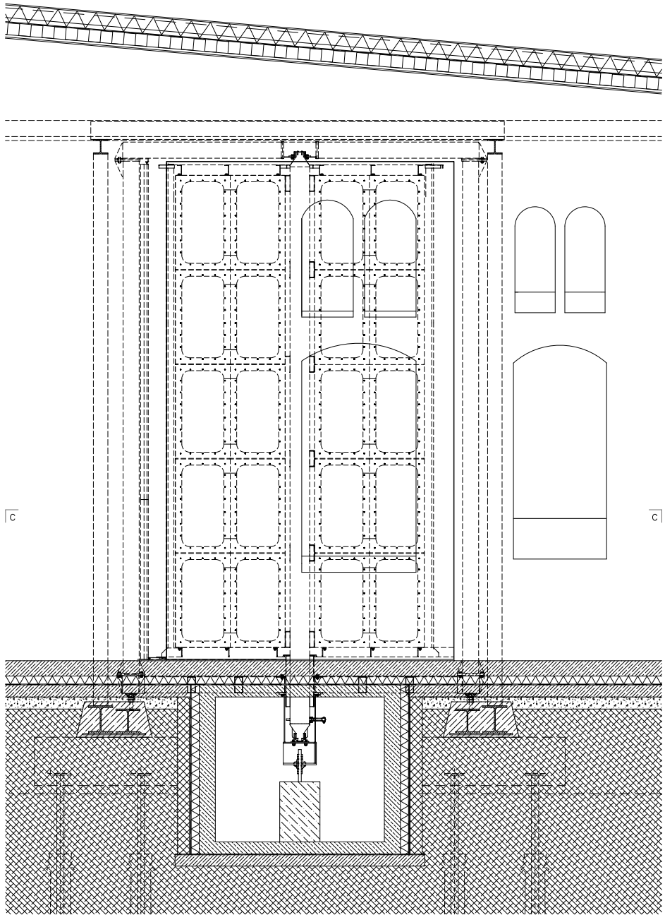
0 1m section A-A
