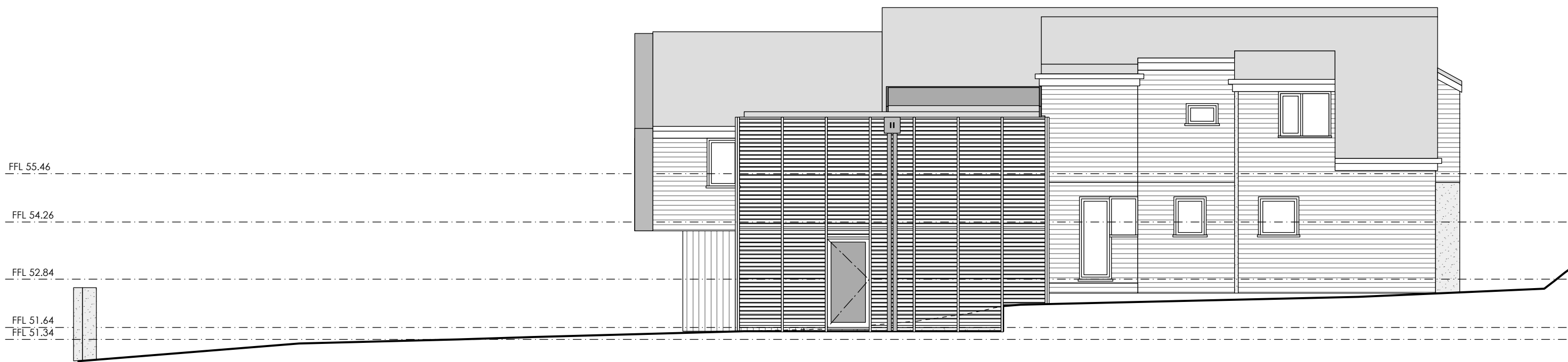
marine parade south east elevation
