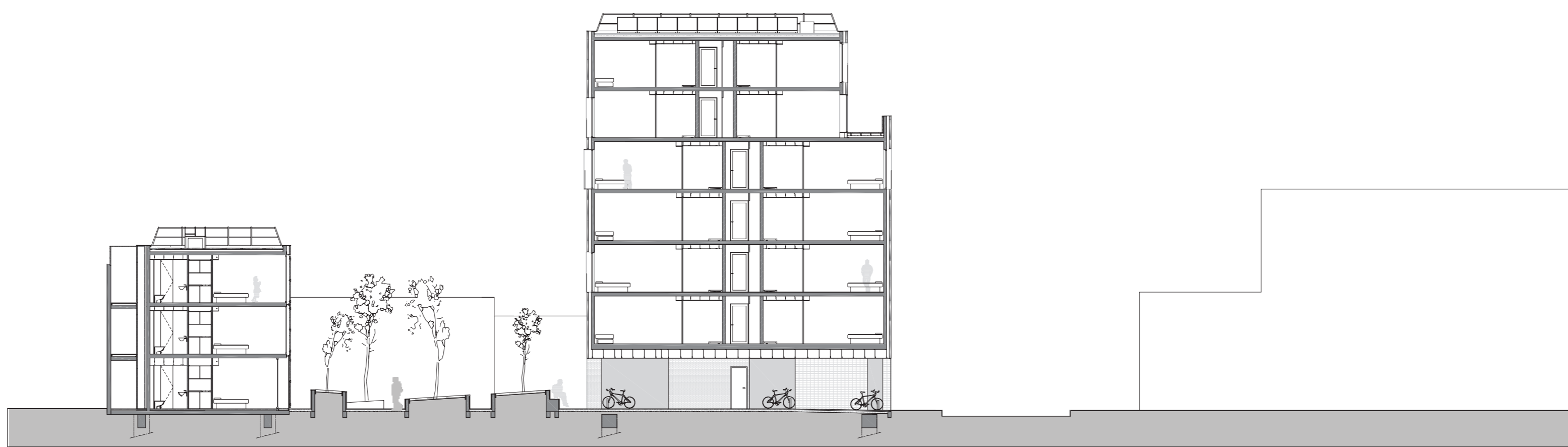
Section CC
