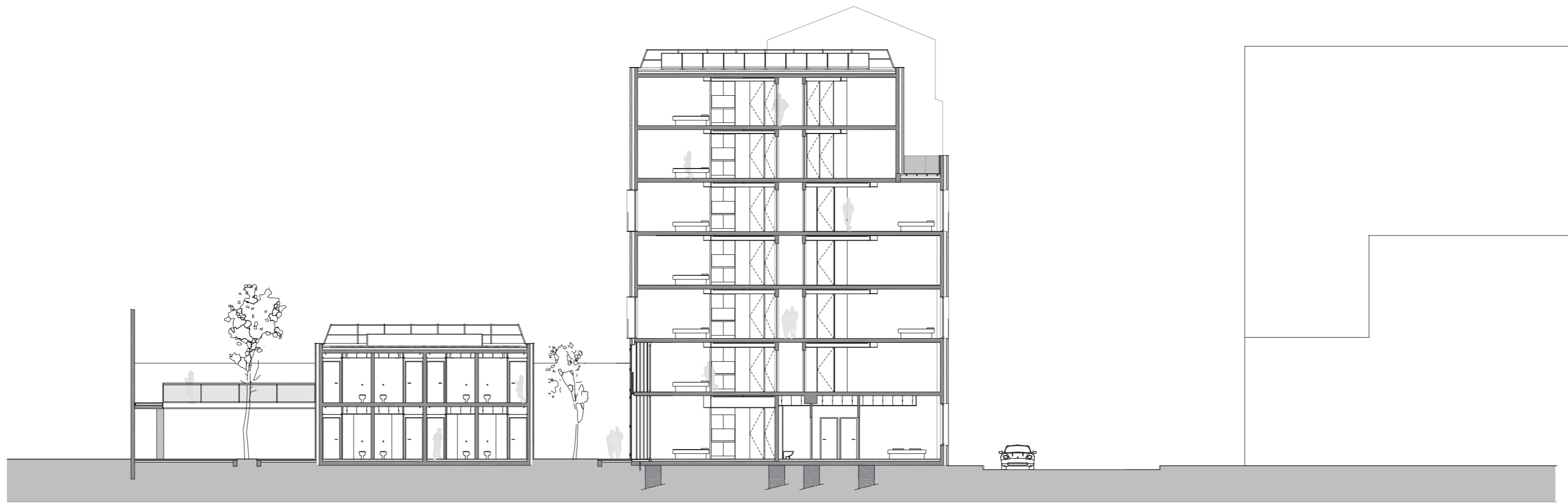
Section BB
