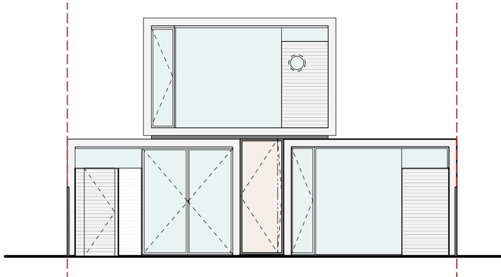
north elevation
