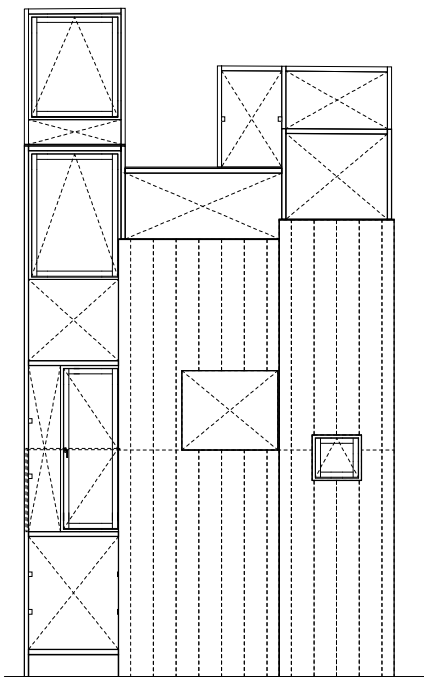
Nouth elevation
