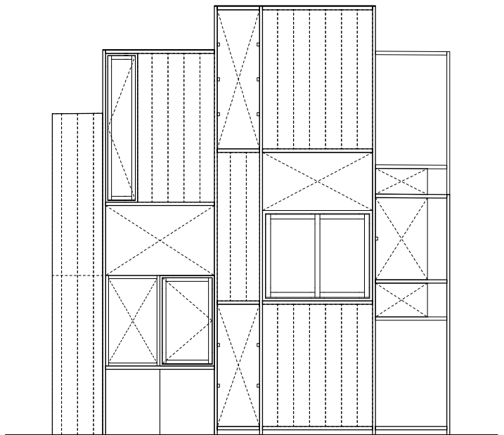
East elevation
