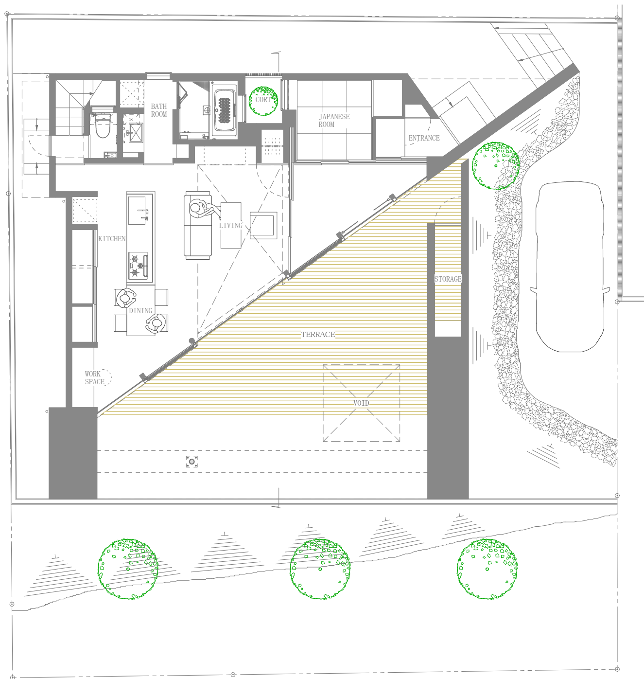
First floor S=1:100
