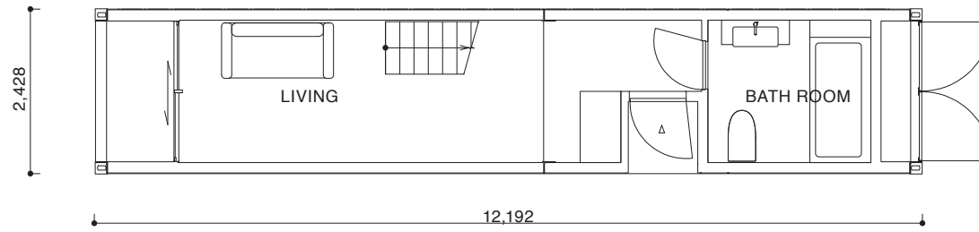
MAISONETTE TYPE 1ST FLOOR PLAN 1/100
