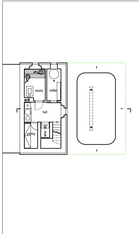
semi basement plan
