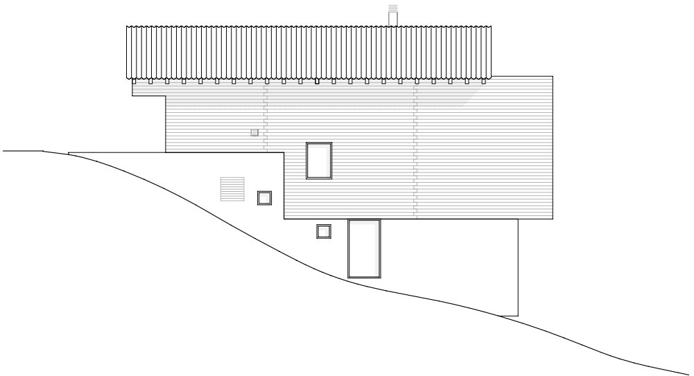
west elevation
