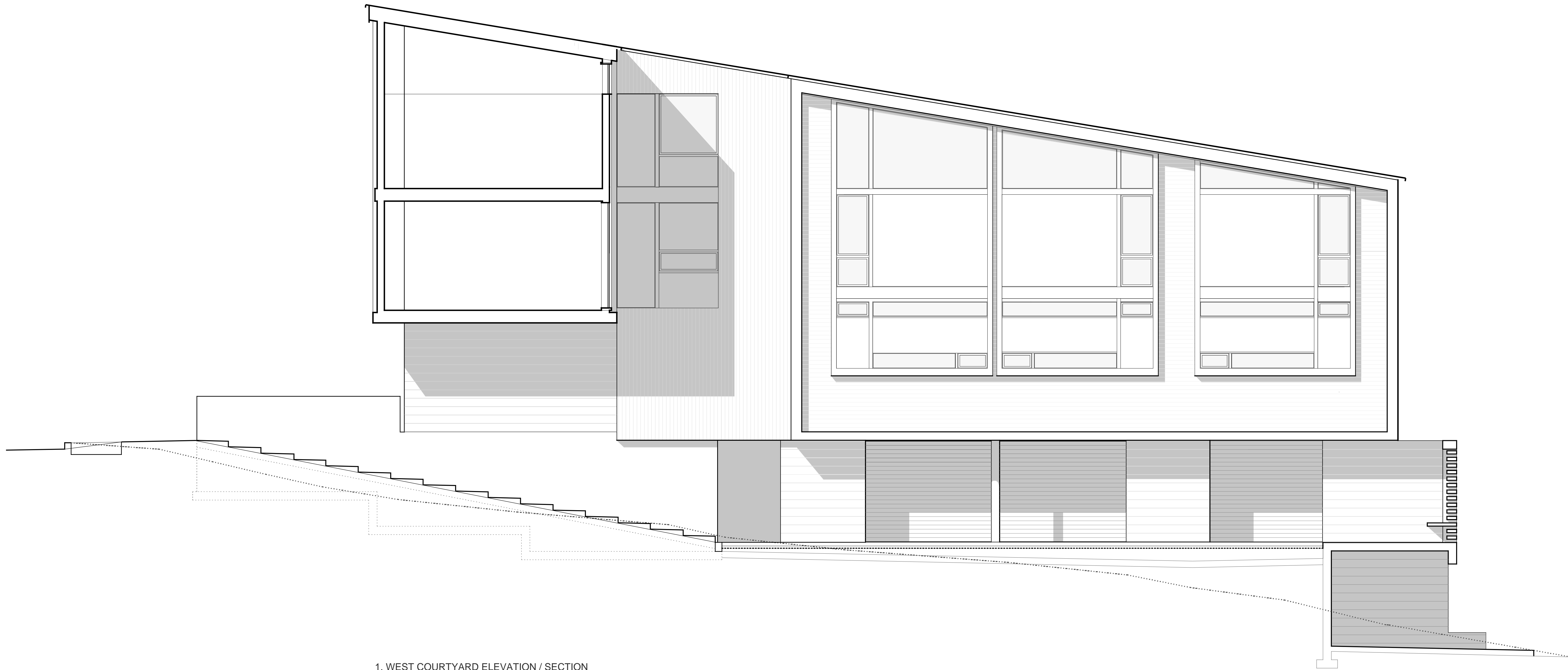
1. WEST COURTYARD ELEVATION / SECTION SCALE 1/4" = 1'-0"
