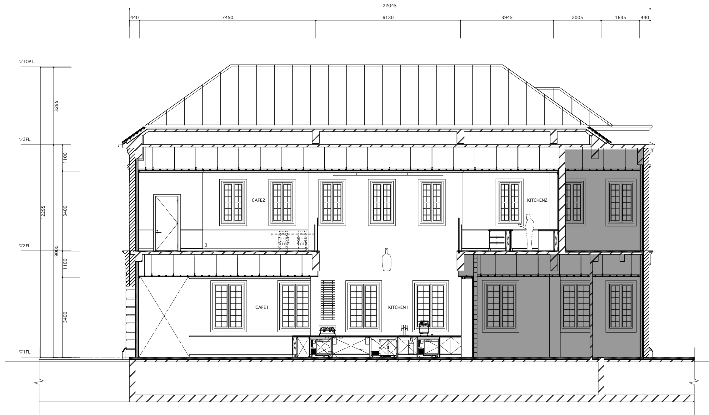
Section_1/100(A3)
