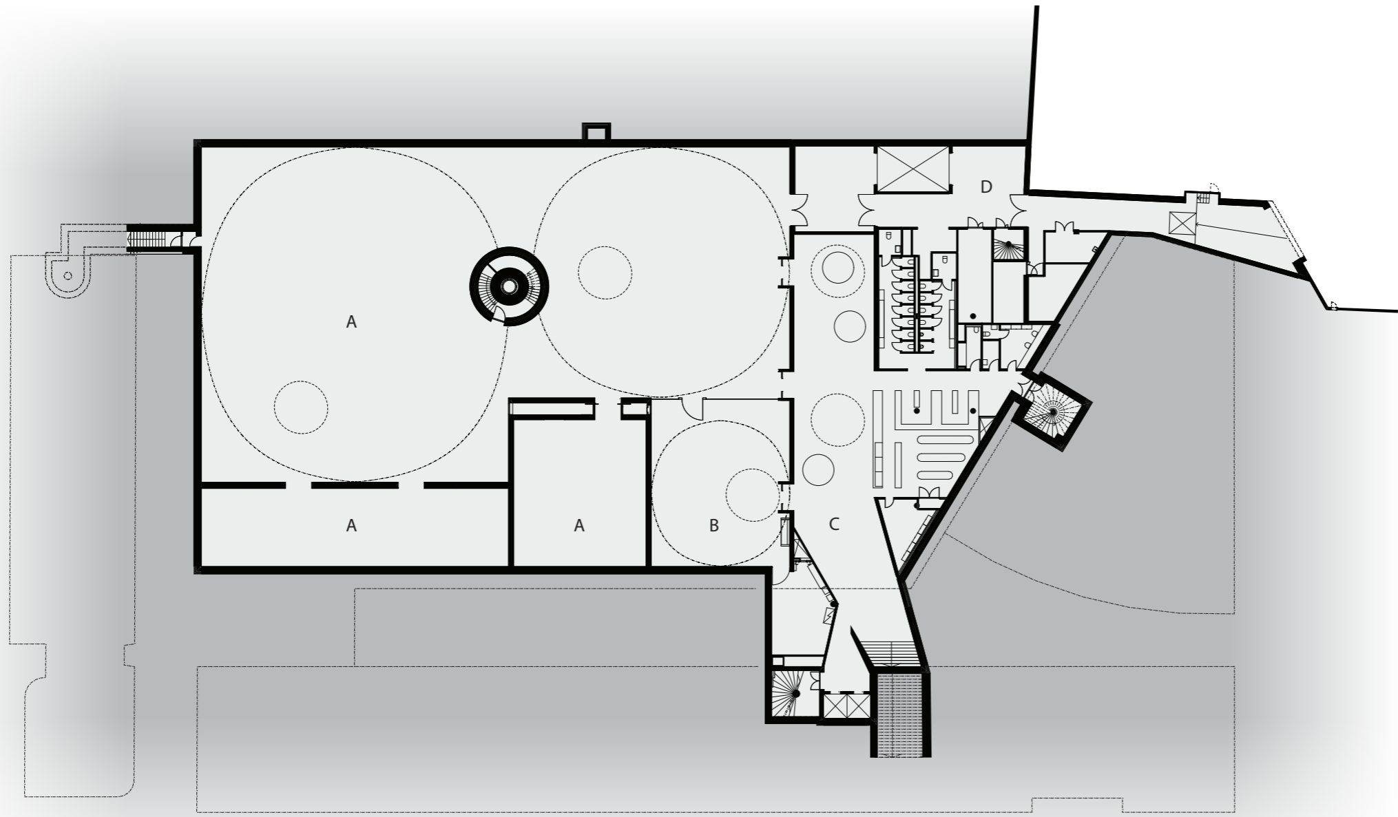
Amos REX -1. Floor 1:500
