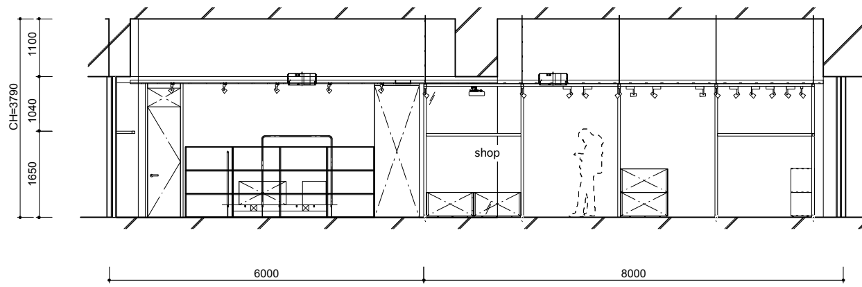
AA' SECTION 1/100
