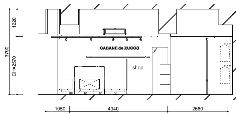
BB' SECTION 1/100
