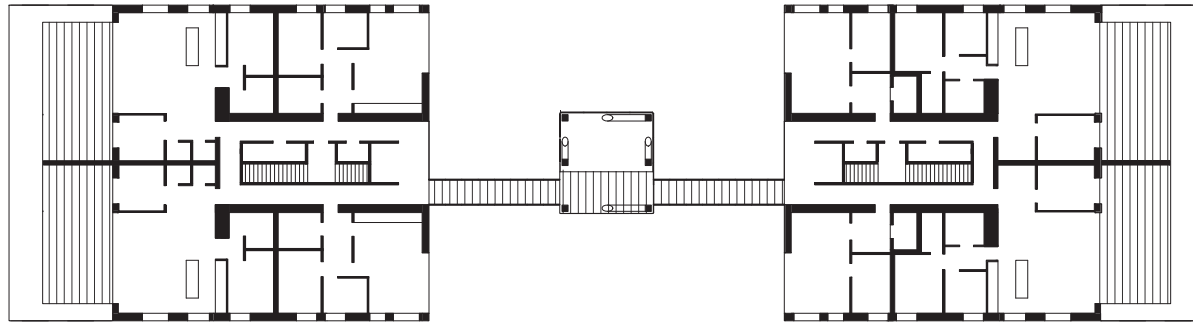
PLAN 11 (HOUSING)
