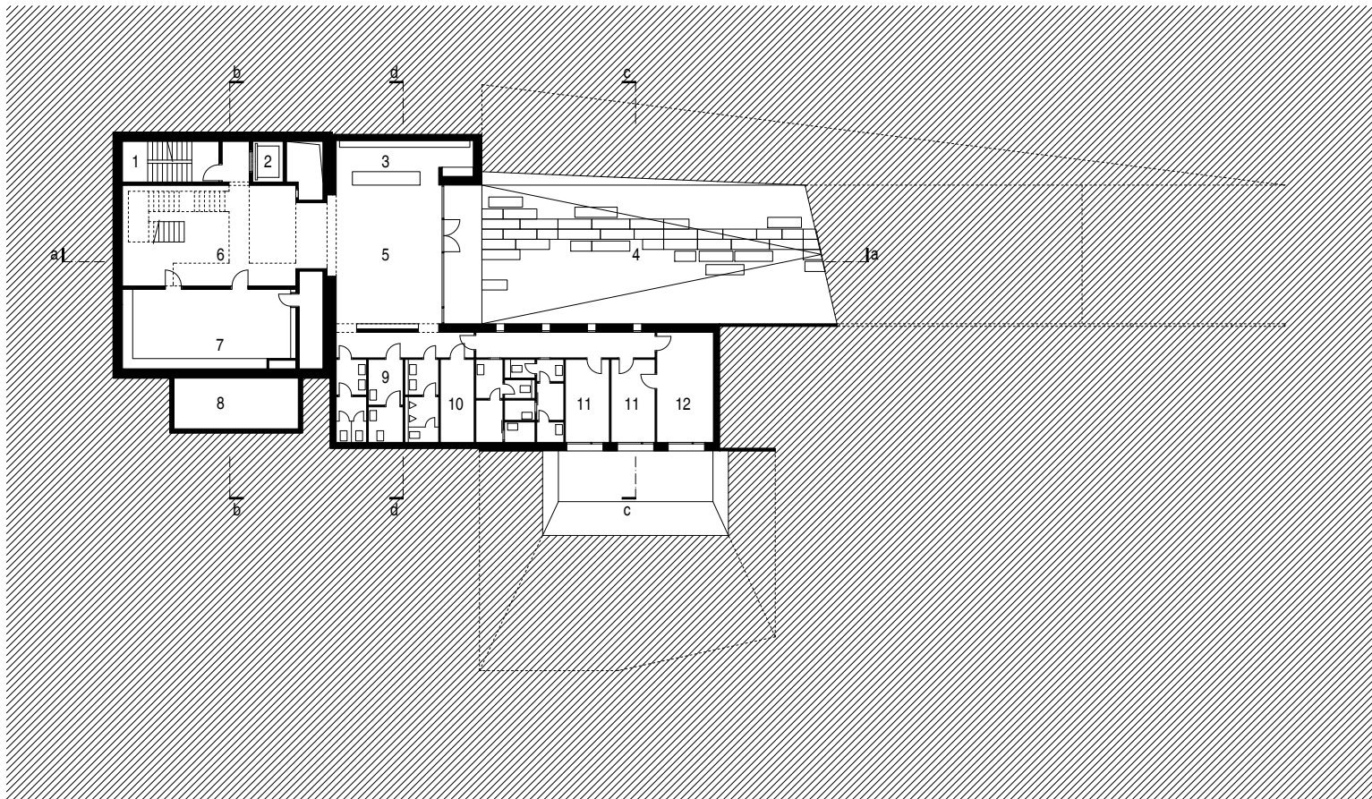
Ground floor plan Scale 1:400
