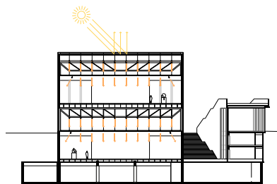
1053_06_D_gallery artificial lighting diagram Gallery artificial lighting © David Chipperfield Architects NO CHARGE
