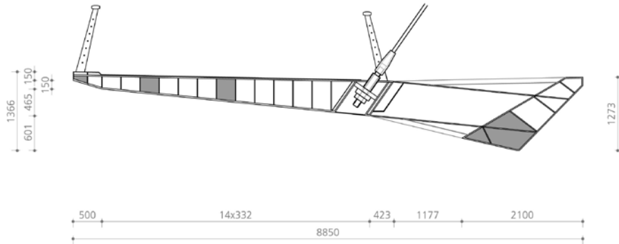
Fig. 6 Bridge deck cross-section, with cable anchorage and added concrete visible
