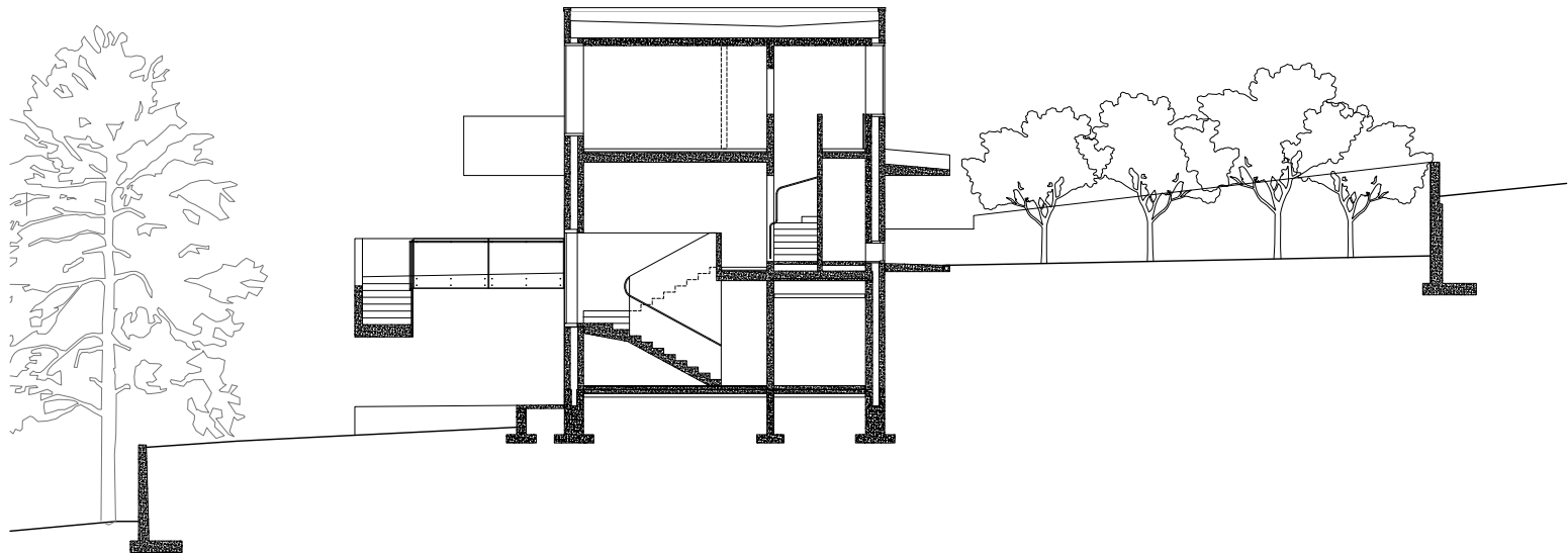
SHORT SECTION 1:200/A4
