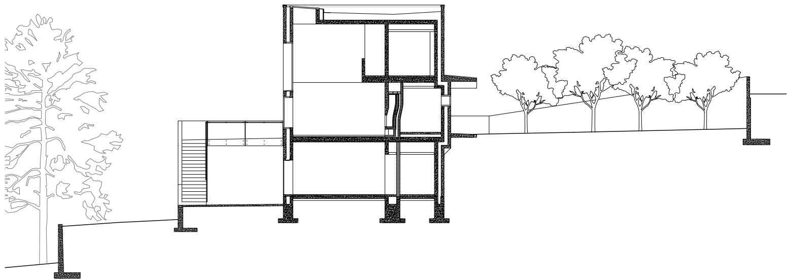
LONG SECTION 1:200/A4
