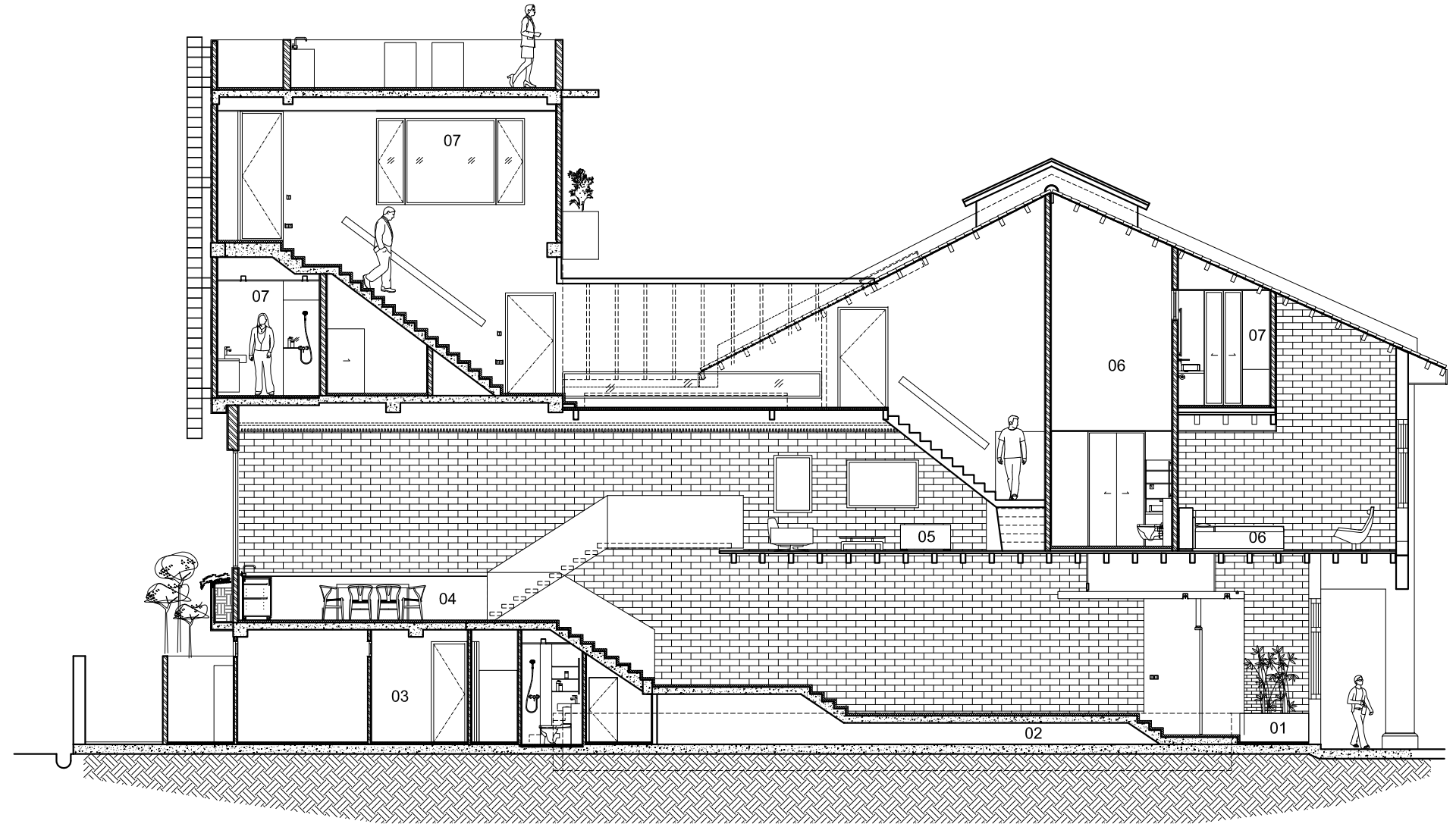
SECTION
