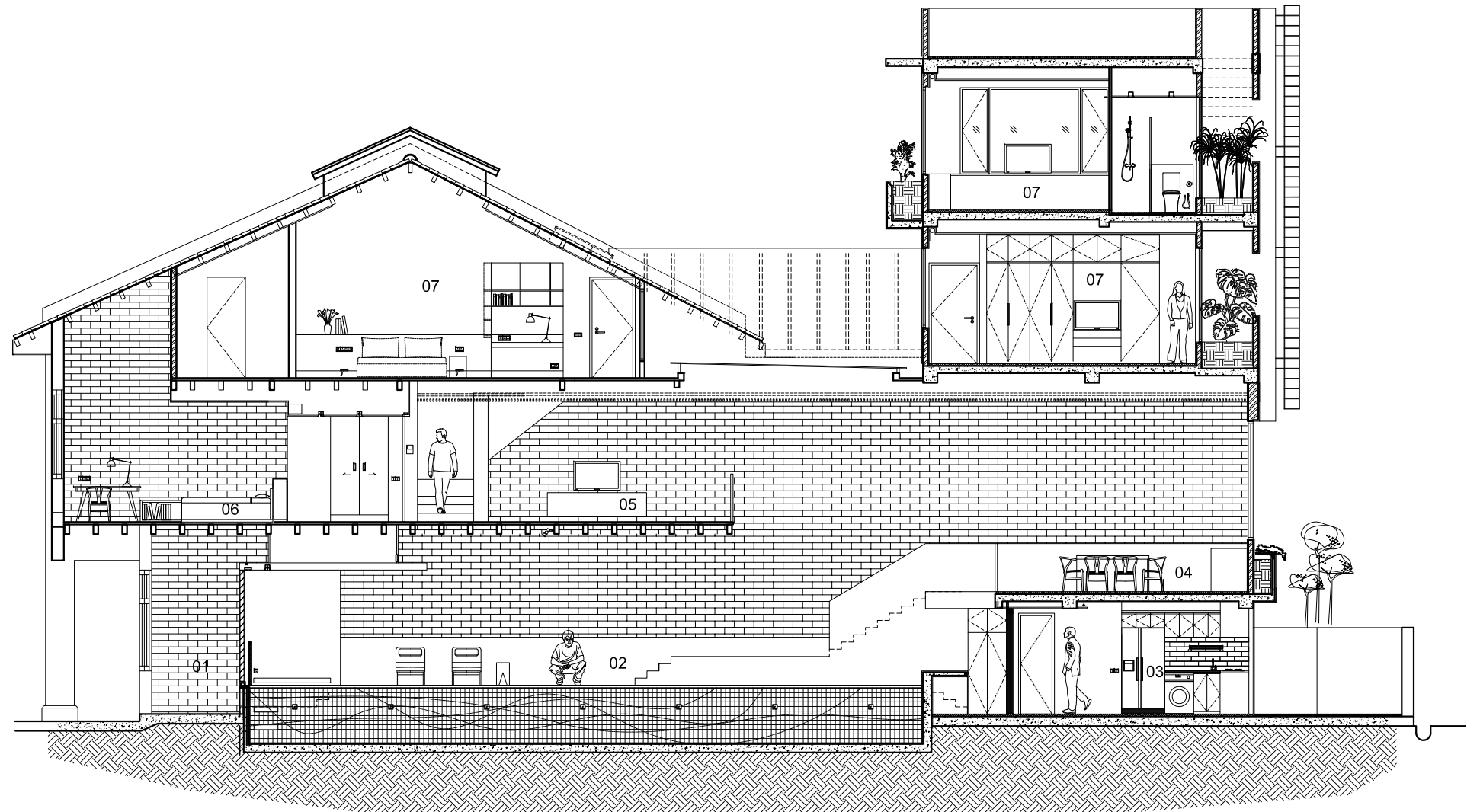
SECTION
