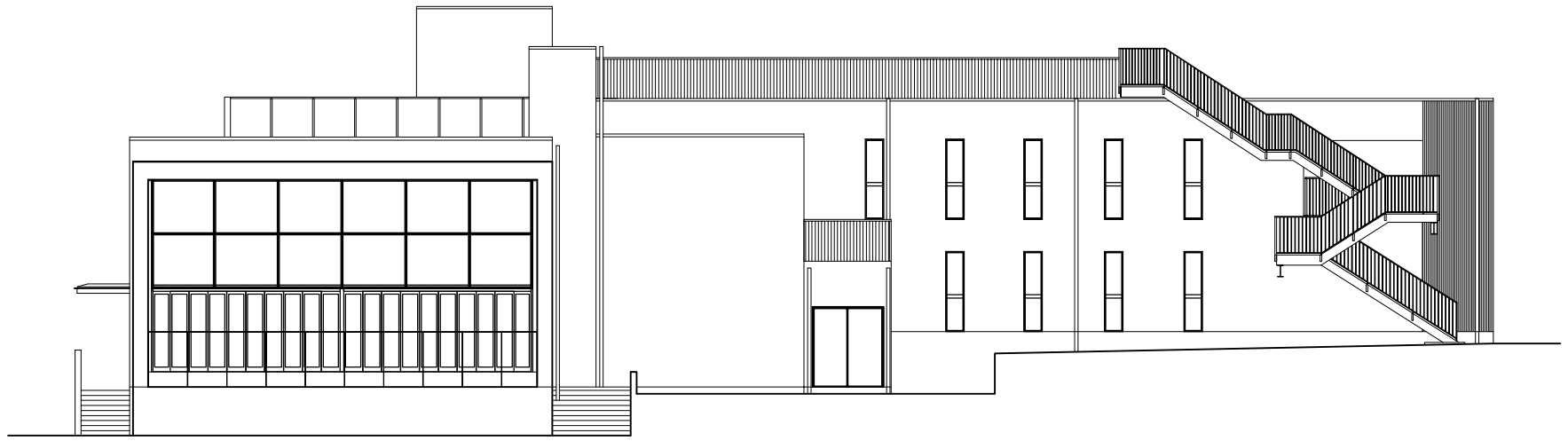
west elevation
