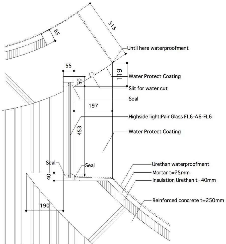
Detail S=1:10 Highside Light
