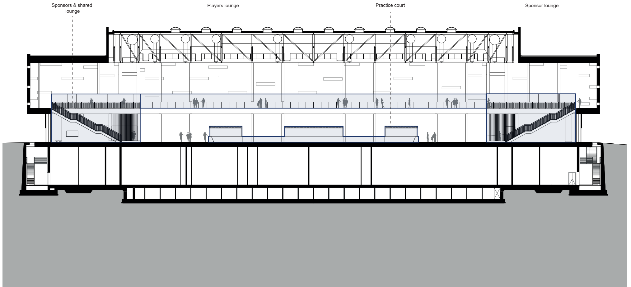
NITTO ATP FINALS - Pala Alpitour trasversal section
