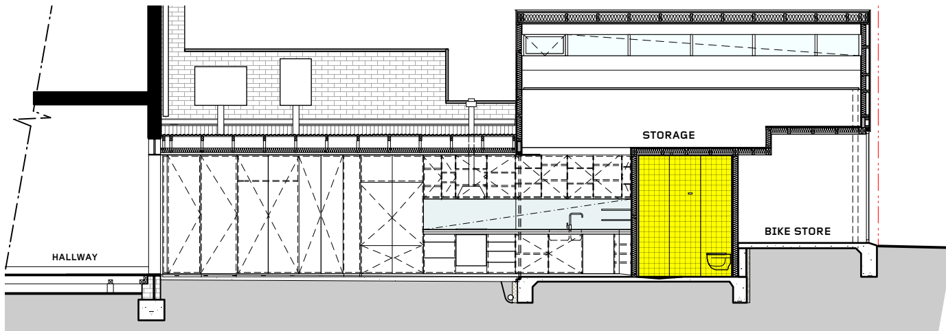
long section
