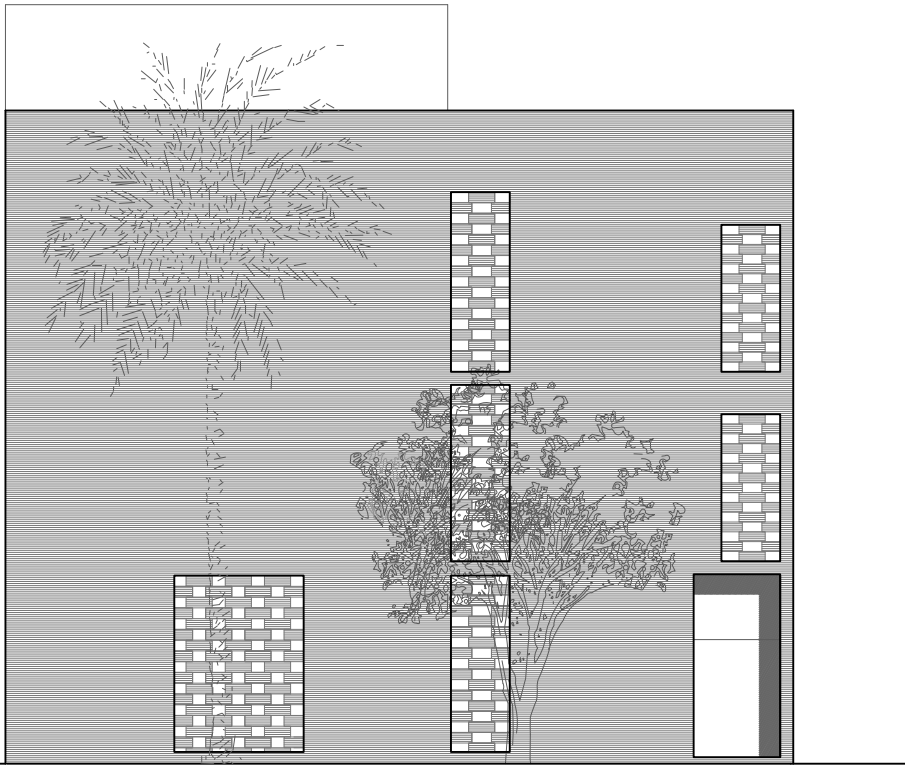
SOUTH ELEVATION.
