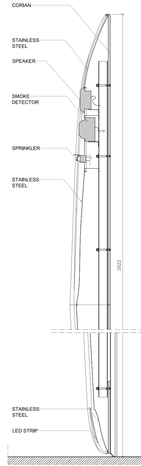
SIDE ELEVATION
