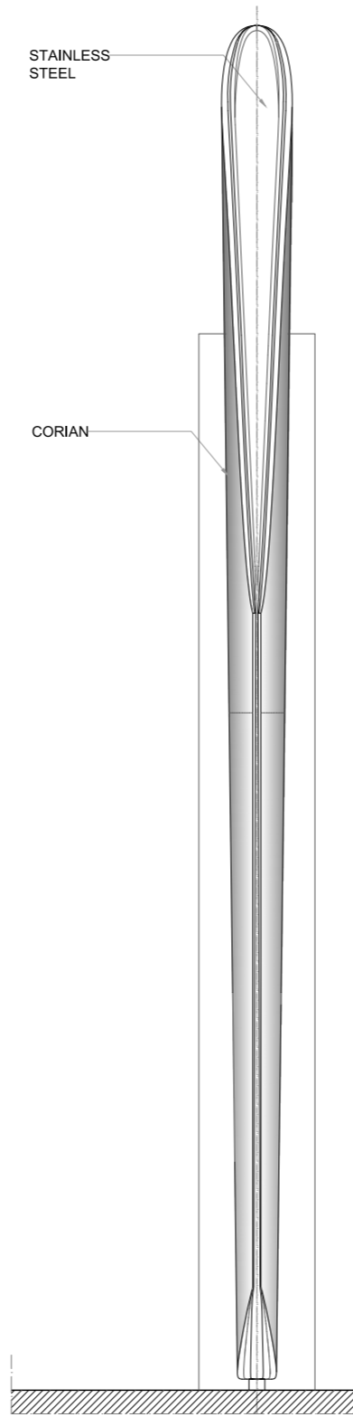
FRONT ELEVATION
