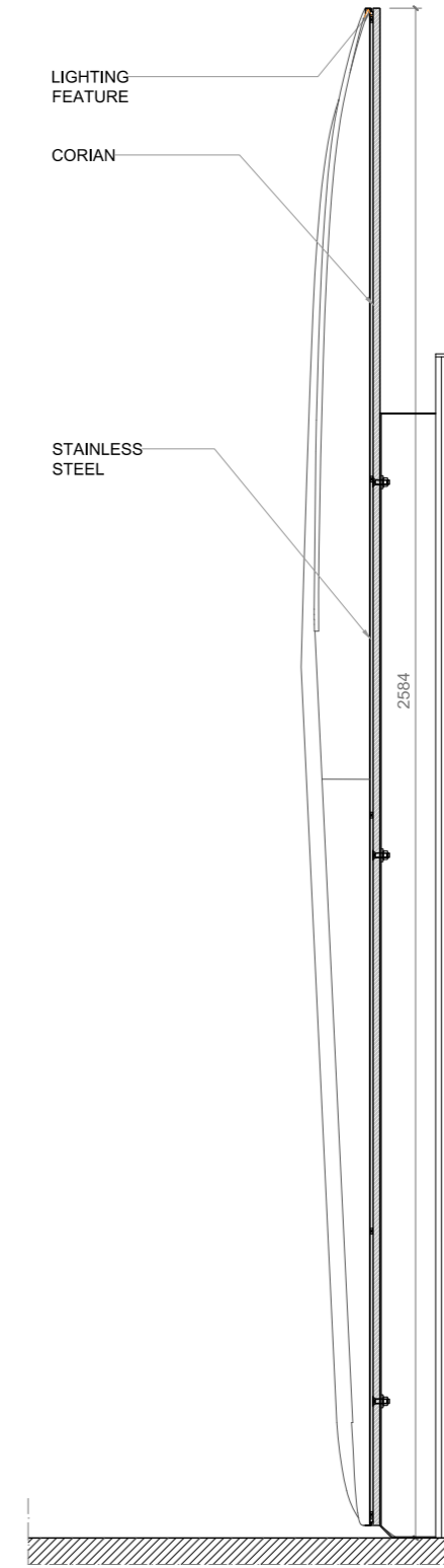
SIDE ELEVATION
