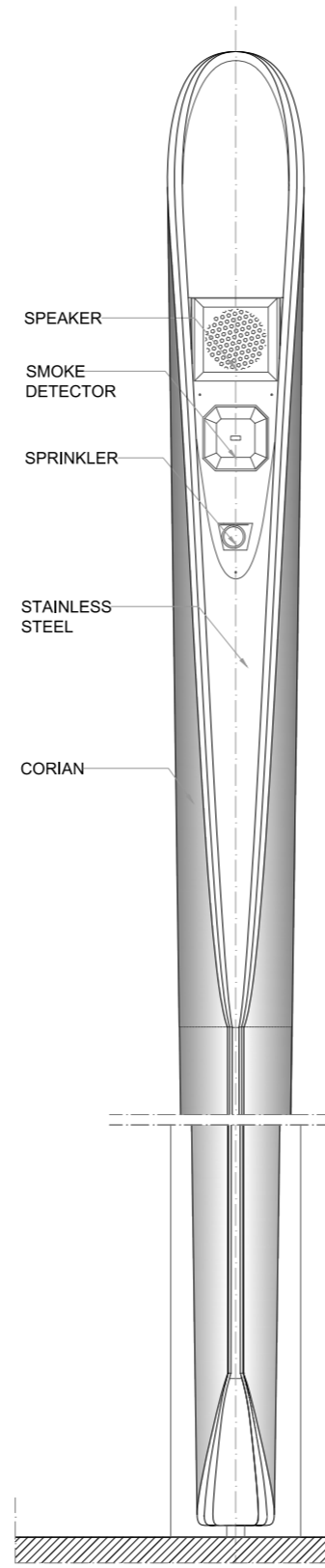
FRONT ELEVATION
