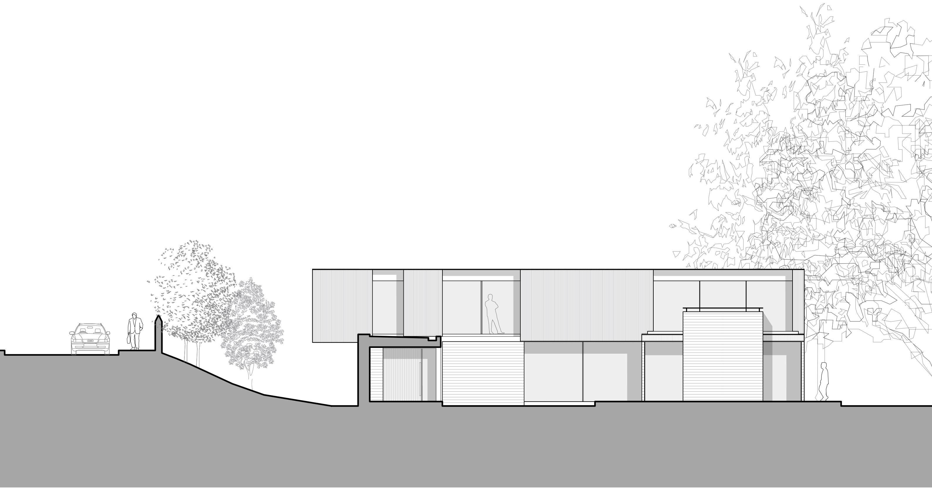
South Elevation
