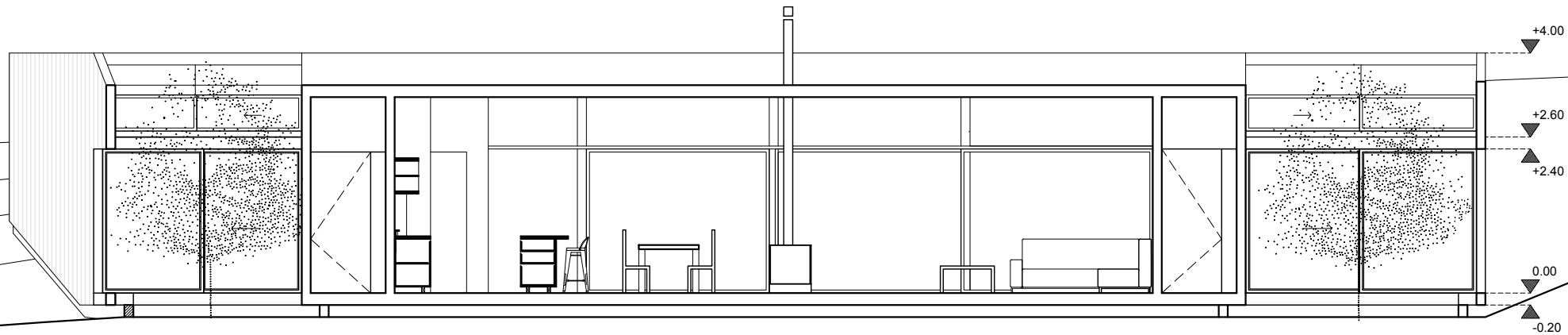
SECTION C-C
