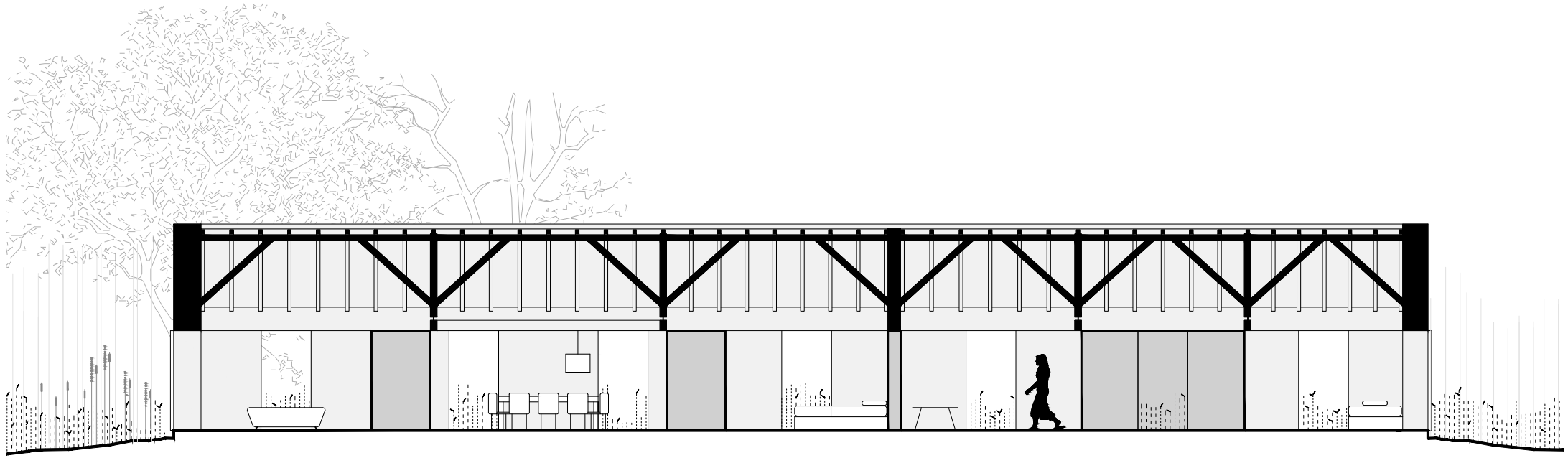
SECTION AB
