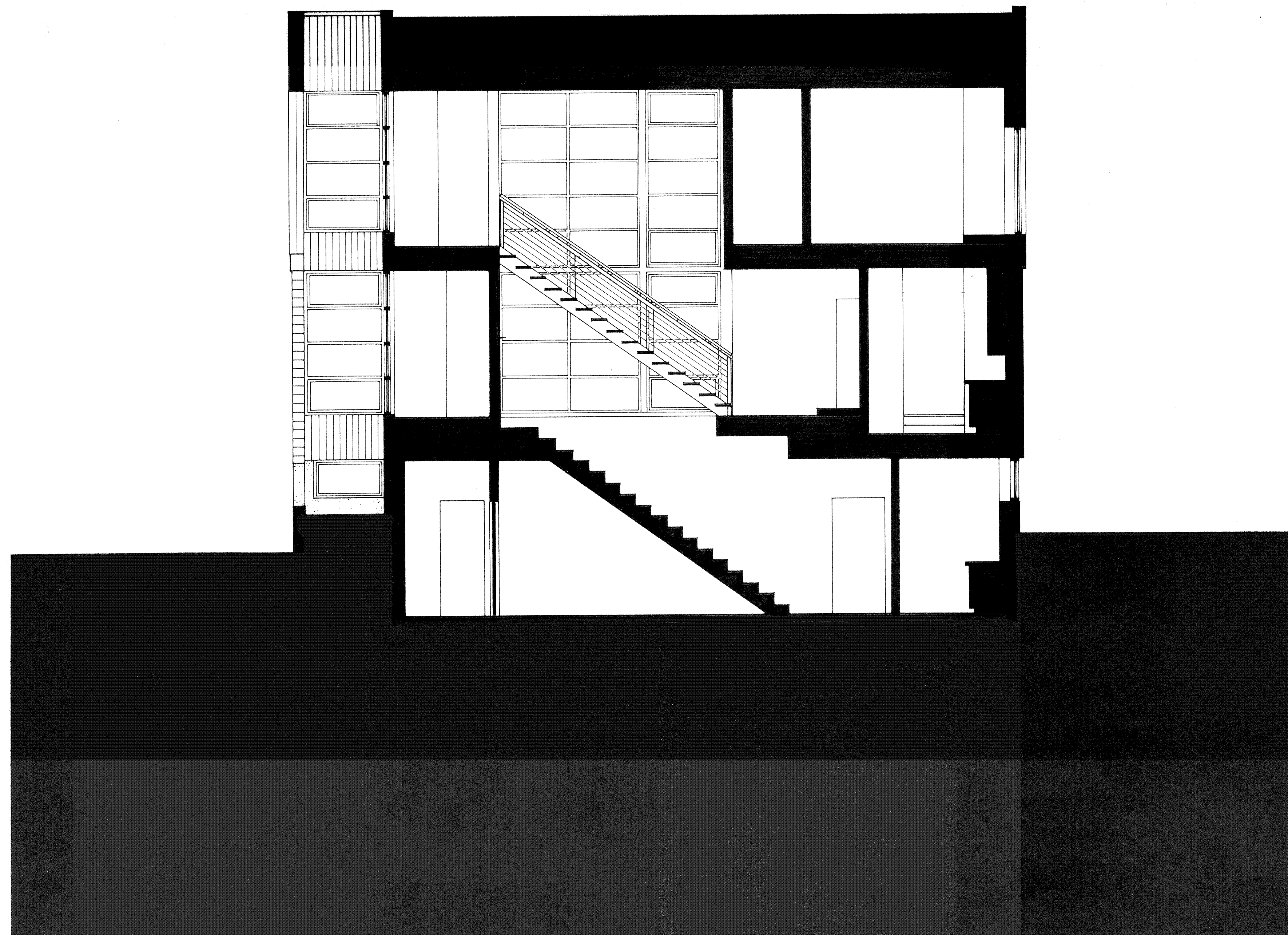
E-W SECTION 0 5 10
