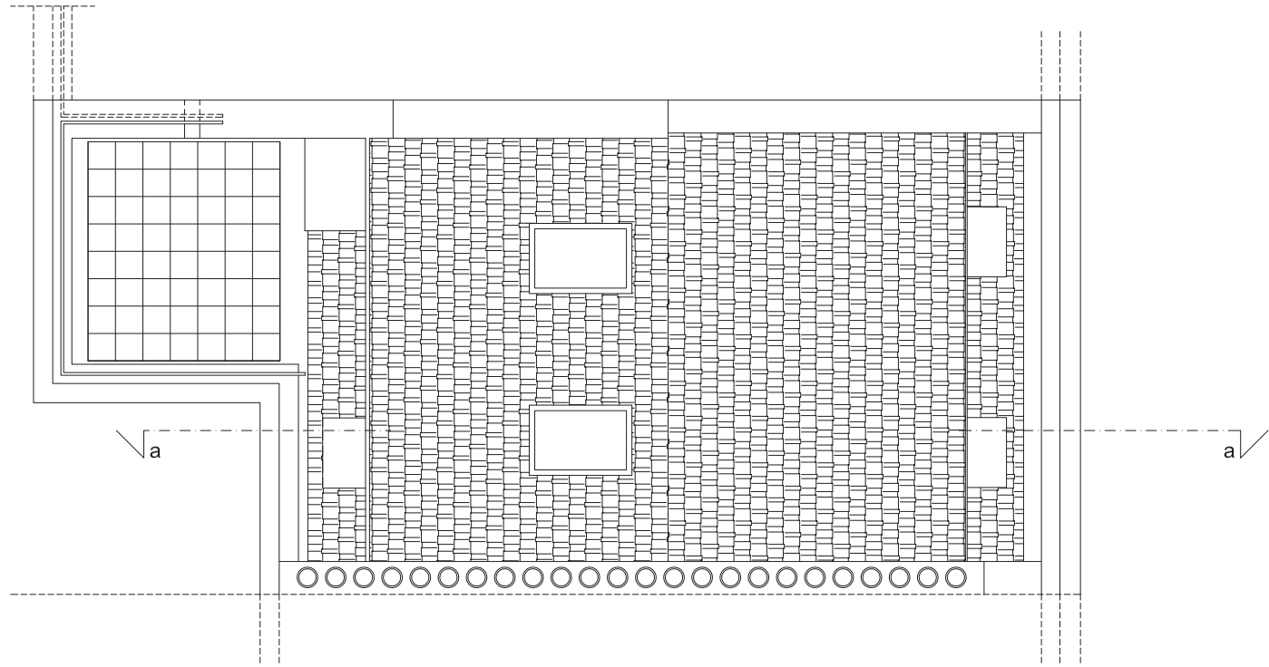
Roof Plan (before the works) scale 1:100
