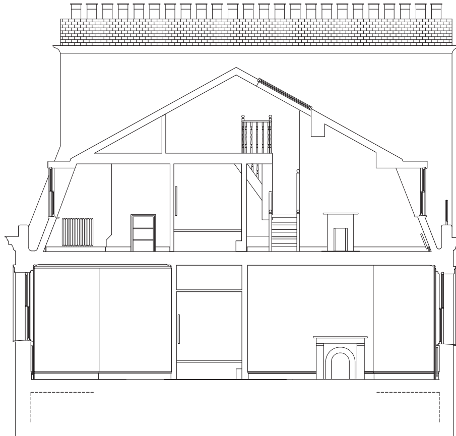
Section a-a (before the works) scale 1:100
