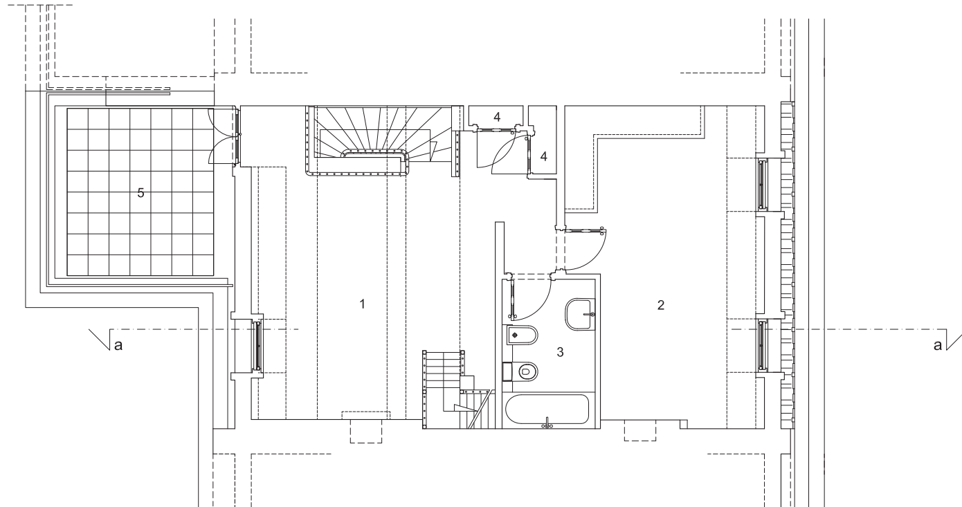
Fourth Floor Plan (before the works)
