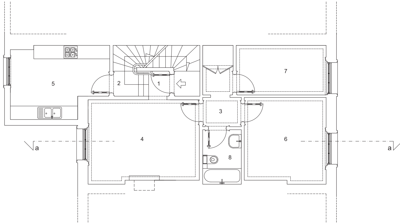
Third floor plan (before the works)
